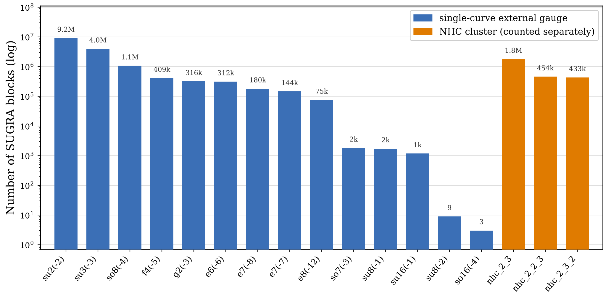
SUGRA blocks containing each external ( \geq 1 )
