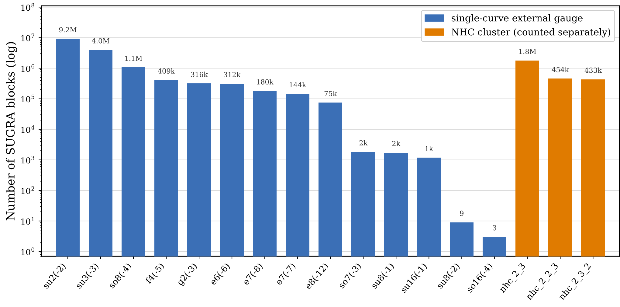
SUGRA blocks containing each gauge algebra ( \geq 1 )
