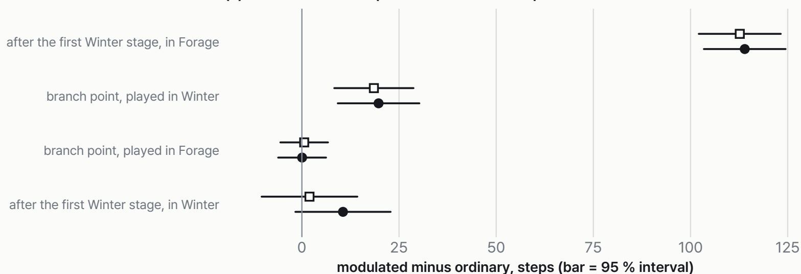
(c) re-check with sampled actions: P3 checkpoints
