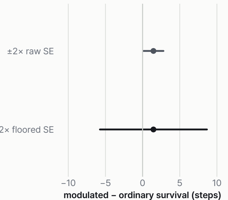
difference +1.46 steps; raw SE 0.67, floored SE 3.60
