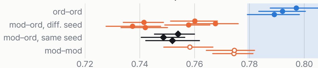
actor.out: (c) different processing, same outcome (same-seed excess E does not hold)
