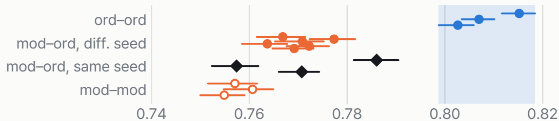
rnn.state: none of the three patterns (undetermined at 3 seeds) (same-seed excess E does not hold)
