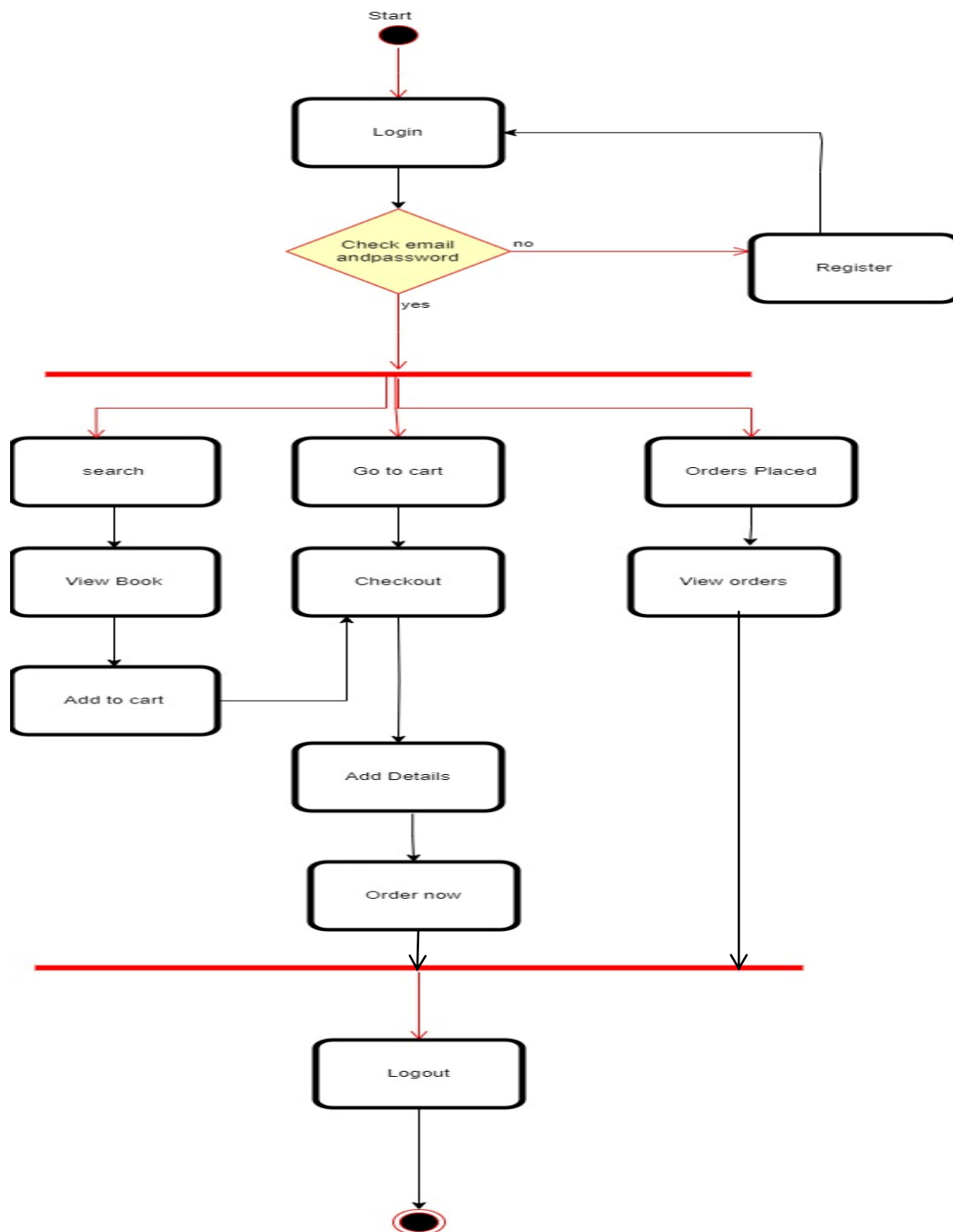
Fig 2.3 Activity Diagram
