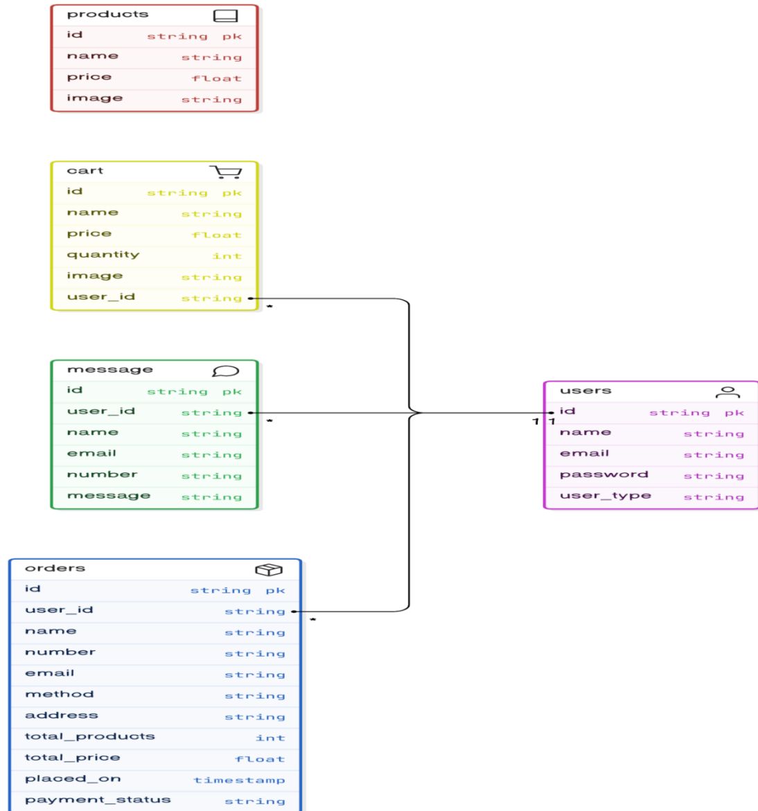
Fig 2.2 Class Diagram
