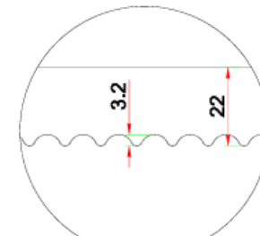
DETAIL 'Y'
