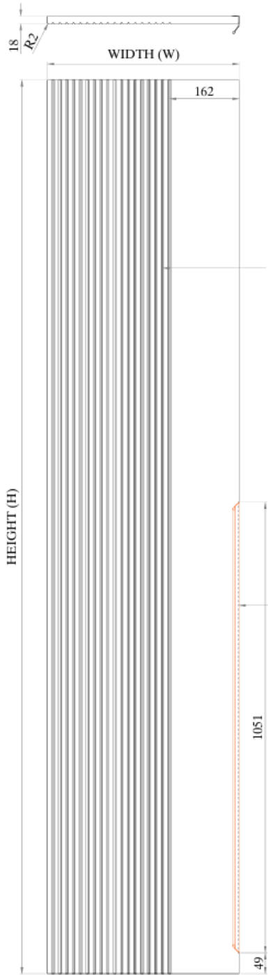
LH SHUTTER
