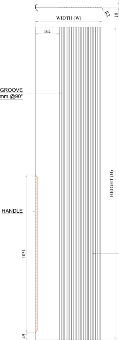
RH SHUTTER
