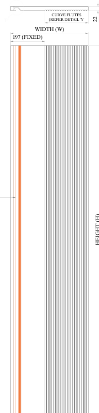
WEDGE-F SHUTTER RH (FINISHED VIEW)
