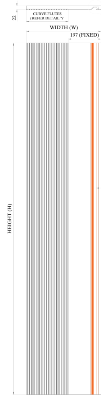
WEDGE-F SHUTTER LH (FINISHED VIEW)
