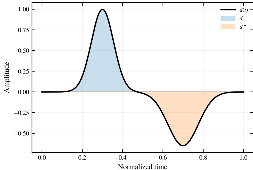
(a) Signed datum and species split
