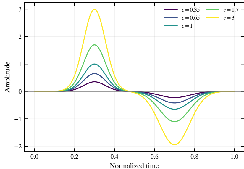
(b) Positive-scale orbit in signal space
