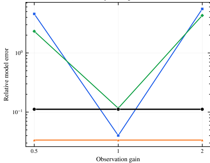
(a) Unknown positive-gain robustness
