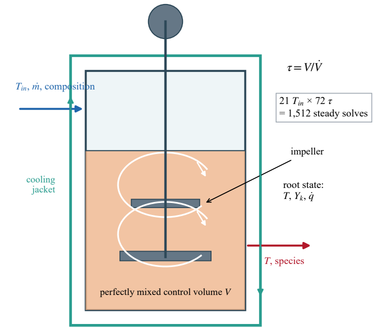
CSTR: well-stirred reactor geometry and coupled thermal balance
