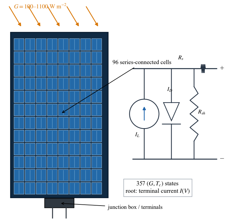
PV module: cell lattice, environmental batch and one-diode solve
