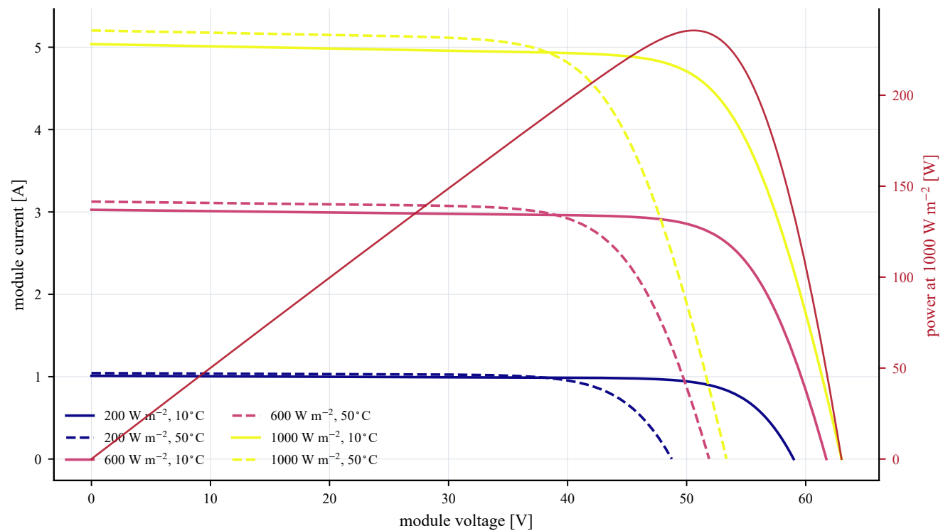
CEC module I-V and P-V curves from pvlb
