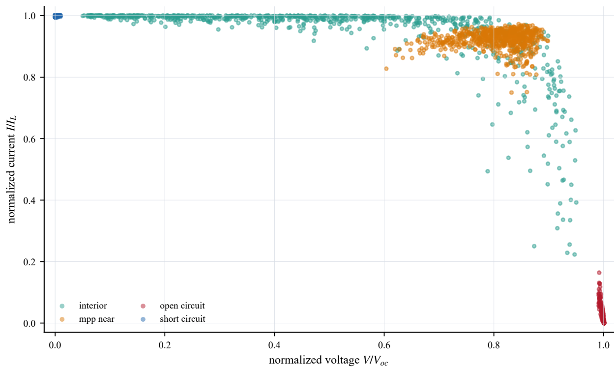
Frozen benchmark coverage in normalized electrical coordinates
