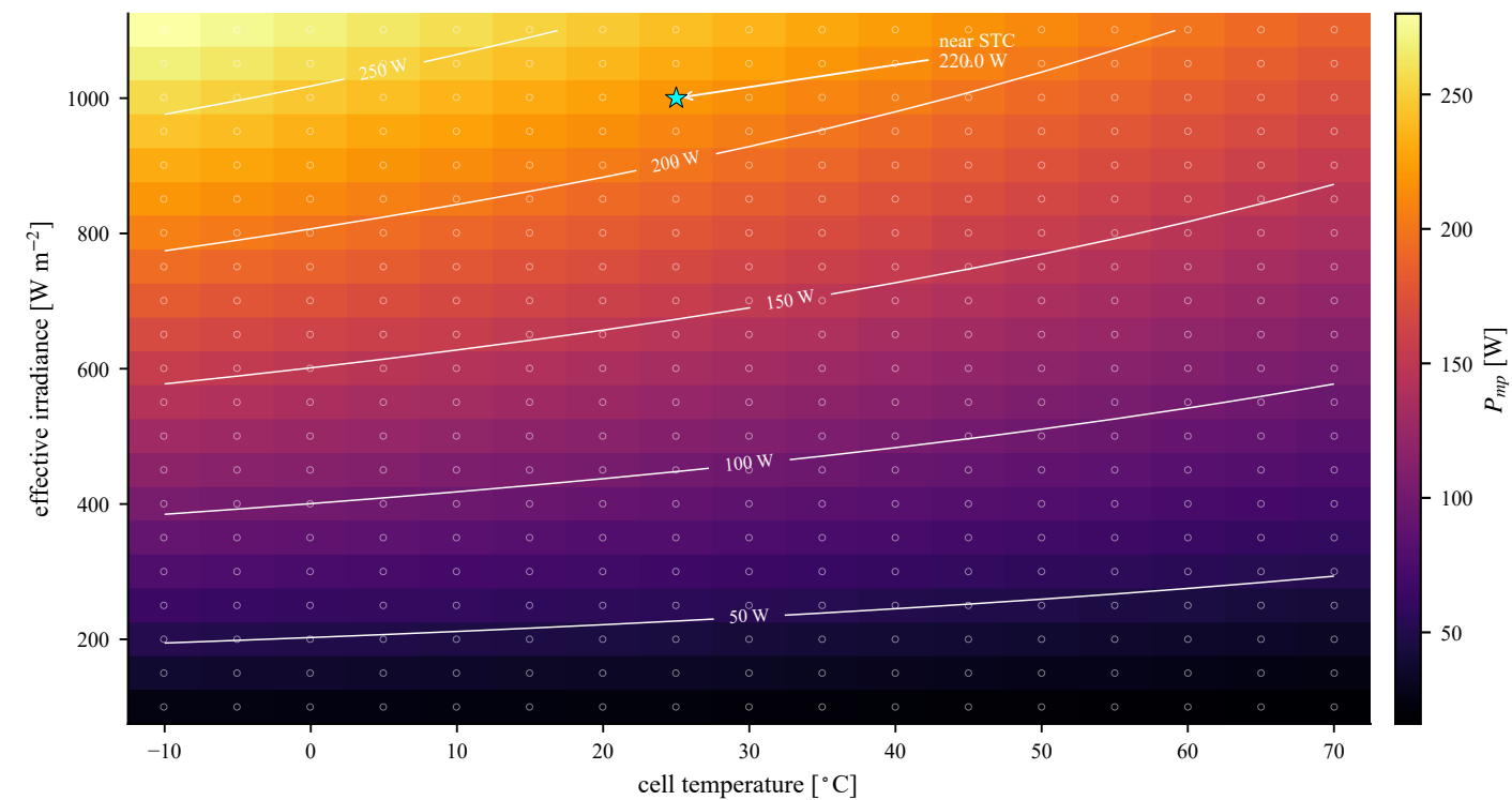
Maximum-power surface: 357 independent operating points
