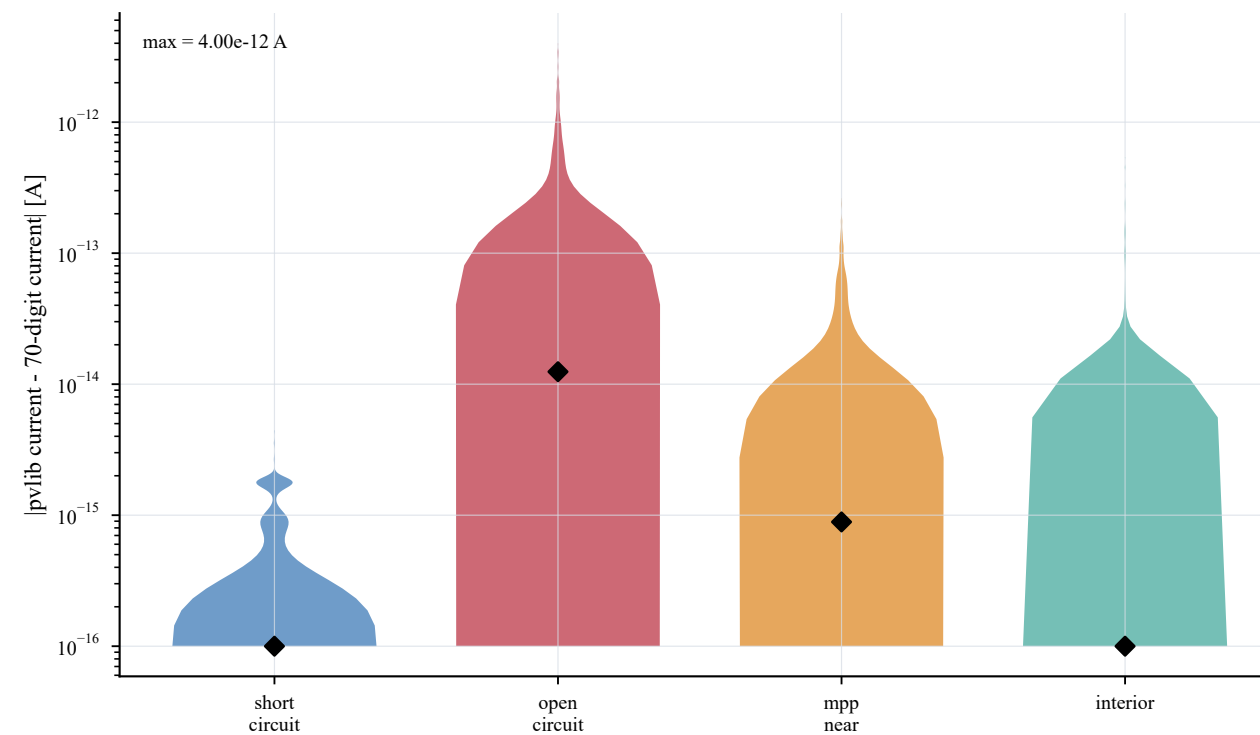
Independent pvlb Brent check against the 70-digit oracle
