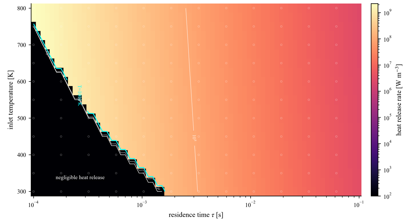
Heat-release field reveals the extinction boundary
