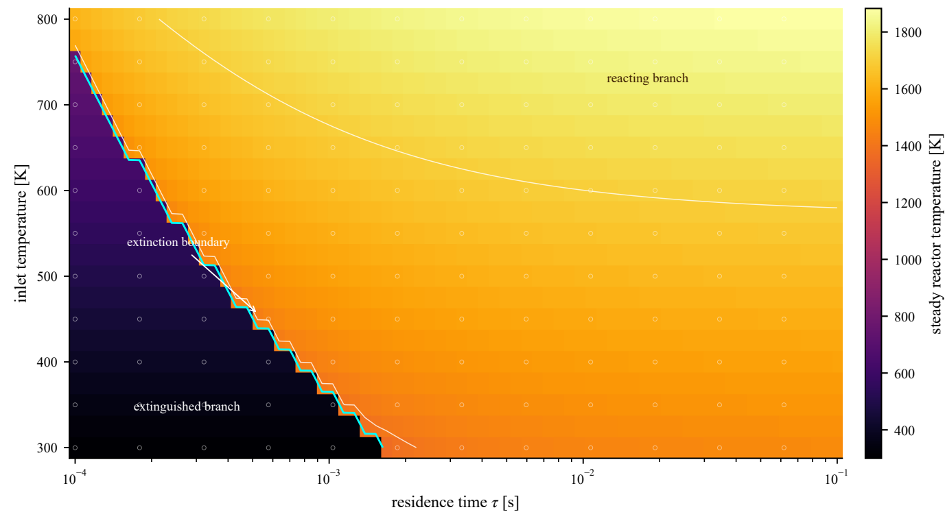
Cantera well-stirred combustor: steady temperature field
