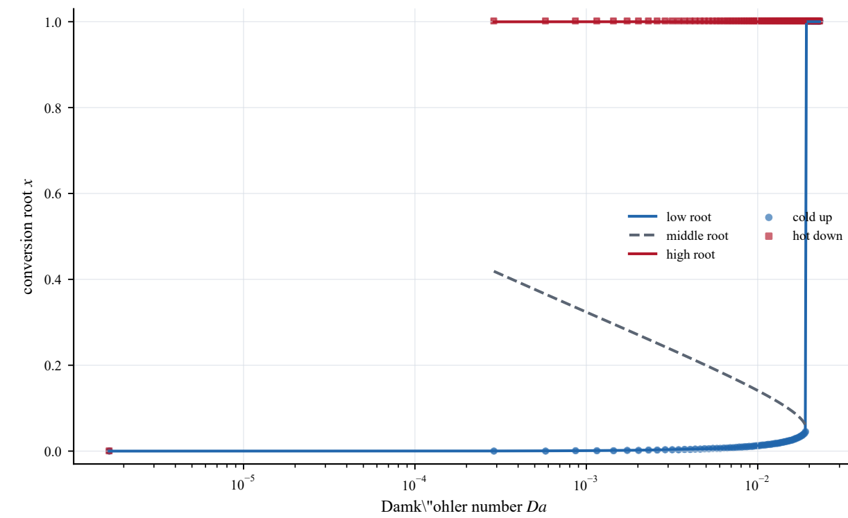
Exact reduced-model folds require branch history
