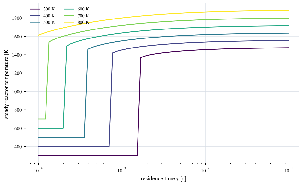
Hot-branch continuation for selected inlet states
