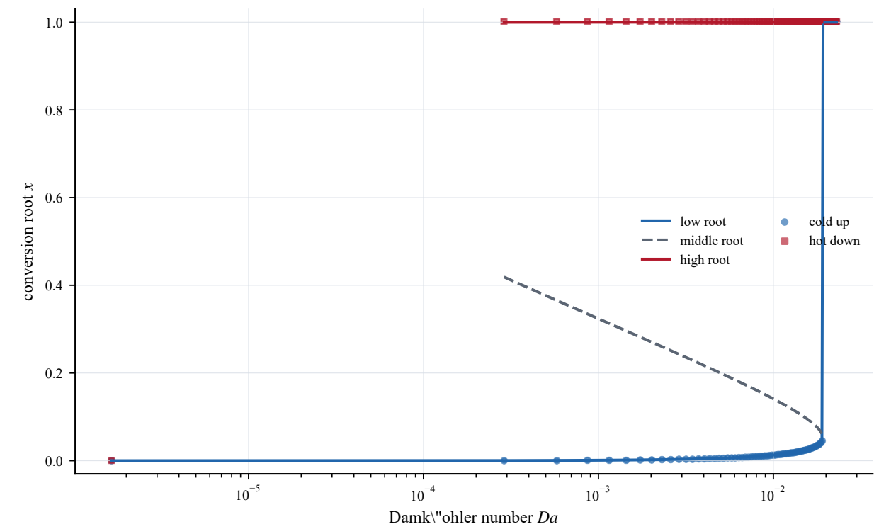
Exact reduced-model folds require branch history
