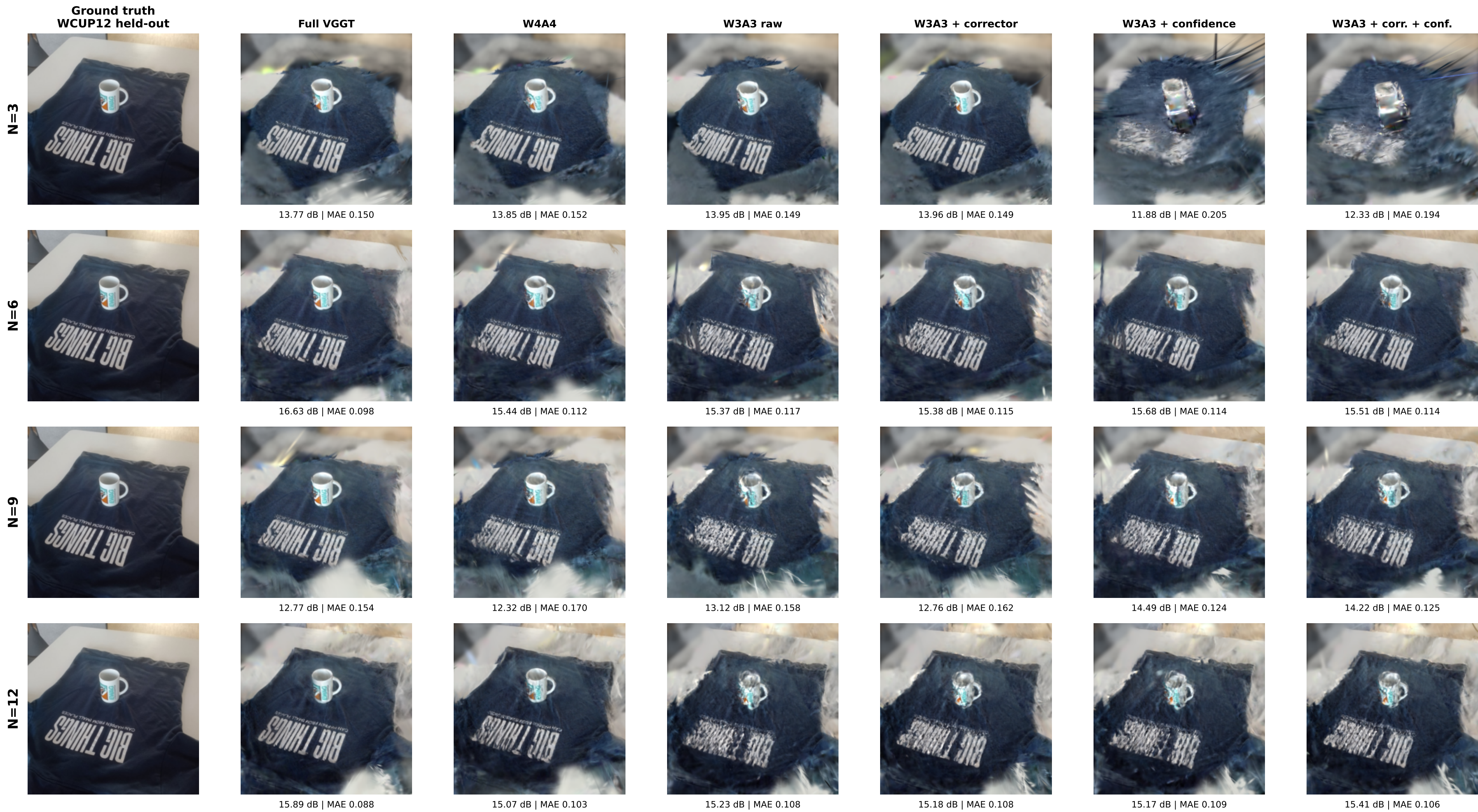
Rows: number of upstream input views. WCUP12 is excluded from 3DGS optimization. Higher PSNR and lower MAE are better.
