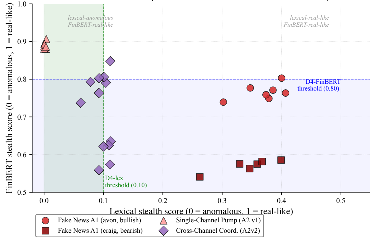
Stealth detector-class dependence: each attack hides in a different blind spot
