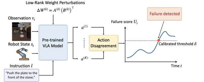
Fig. 1: Overview of the proposed PFD framework. Given the current observation, robot state, and language instruction, low-rank weight perturbations generate local parameter variations around the pretrained VLA model. Disagreement among their action predictions provides an epistemic uncertainty-based failure score U_t . A failure is detected when U_t exceeds the calibrated threshold \delta .
