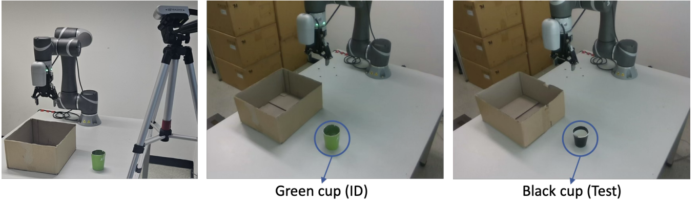
Fig. 5: Real-world setup and evaluation conditions. Left: robot workspace with the TM5-900, AG95 gripper, and fixed RealSense D435i camera. Middle: green-cup ID condition used for reference, calibration, and ablation. Right: unseen black-cup condition used for object-shift testing. Object positions are randomized within the same workspace region.
