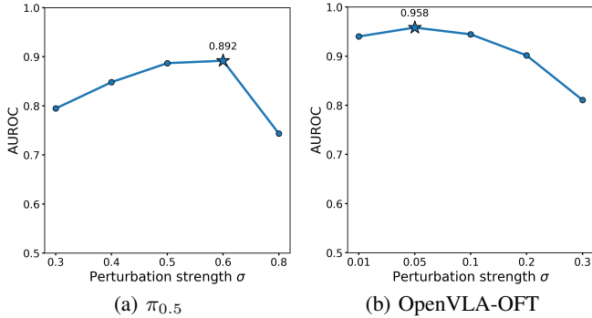
Fig. 4: Sensitivity of failure-detection AUROC to perturbation strength \sigma on LIBERO-10 using K = 2 . Stars indicate the best-performing strength for each model.
