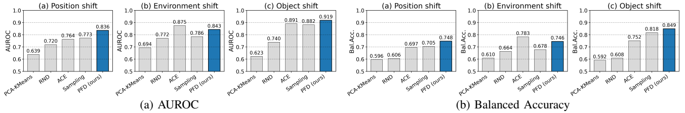
Fig. 2: Failure detection performance averaged across LIBERO-PRO suites within each distribution-shift category. PFD is highlighted in blue, while baseline methods are shown in gray.
