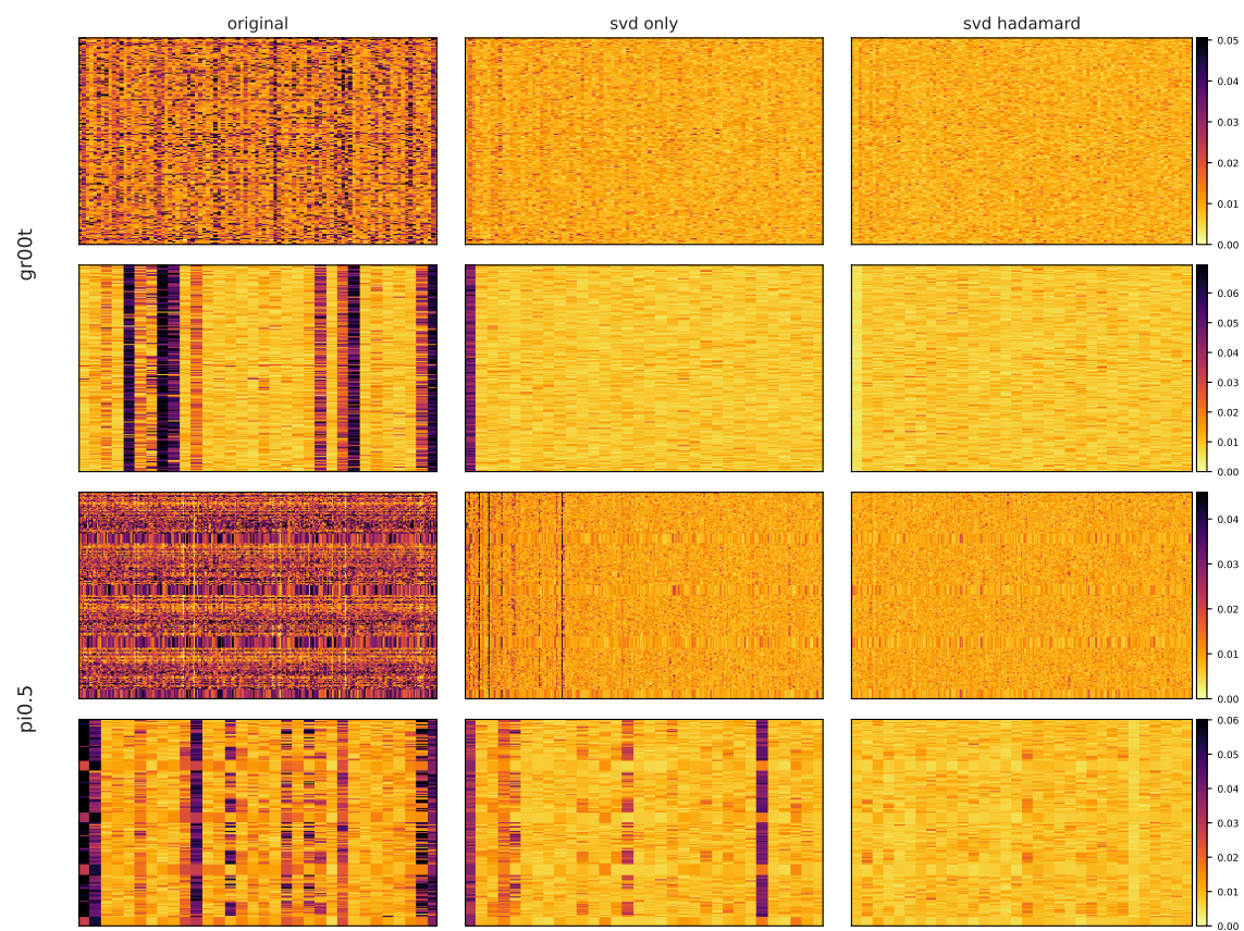
Figure 9: The quantization error with different rotation methods.
