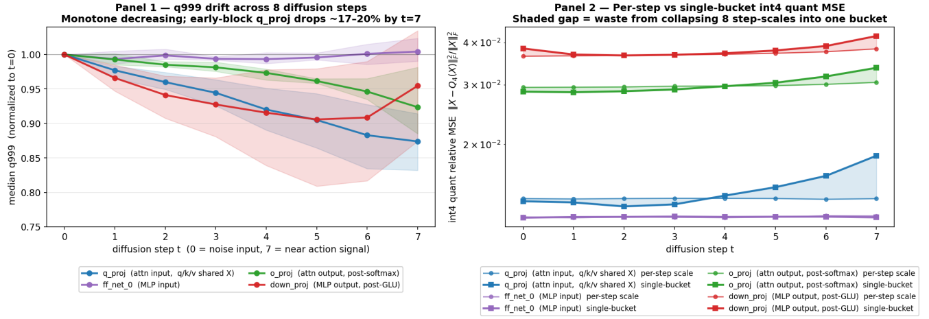
Figure 7: Necessity of per-step act_scale on the DiT side. Left: per-channel q999 across the 8 Euler denoising steps for four DiT layer kinds (normalized to t = 0 ). Right: int4 quantization MSE per step under a step-specific scale (circles) vs a single-bucket scale (squares); shaded area = waste from collapsing 8 step-scales into one. Time-conditioned magnitude drift only appears at layers reading the AdaLayerNorm output (attention QKV projections), and per-step scaling helps exactly those layers.
