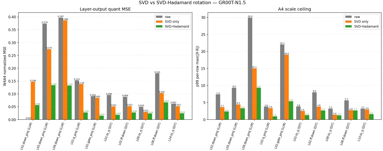
Figure 6: Per-layer W4A4 quantization quality on GR00T-N1.5. Left: normalized MSE between FP16 and W4A4 layer outputs. Right: 99th-percentile per-row max of rotated activations (sets the A4 scale ceiling). Bars compare raw, SVD-only, and SVD-Hadamard (A2-lite) rotation across 5 LLM + 5 DiT sampled layers. SVD-Hadamard yields the lowest nMSE and lowest scale ceiling on 9/10 layers. The single exception is LLM.L02.down_proj, whose extreme channel-skew ( \approx 50000\times ) aligns with the SVD basis and is only partially mitigated by the within-block Hadamard mixing.
