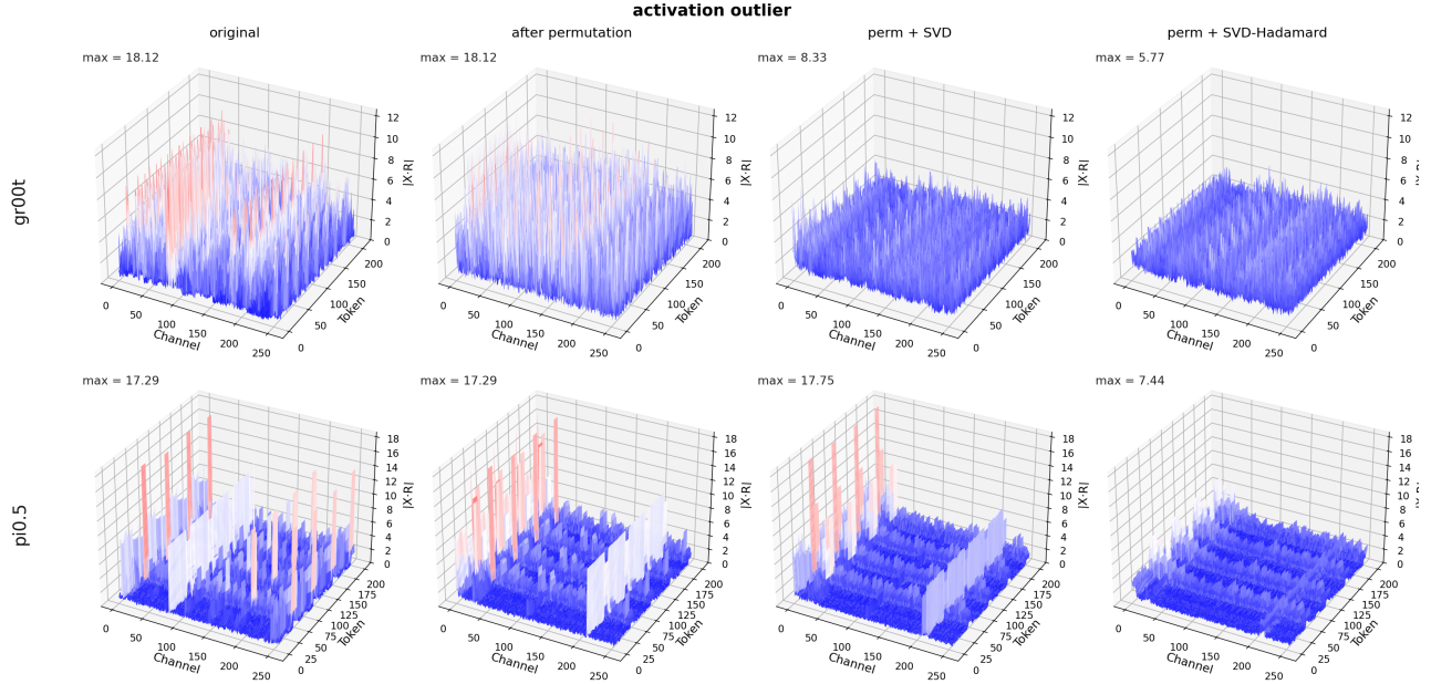
Figure 3: Outlier suppression with QuantVLA (Zhang et al.) and our SVD-Hadamard. We visualize per-token, per-channel magnitudes |\mathbf{X} \cdot \mathbf{R}| for representative layers of GR00T-N1.5 (top) and Pi-0.5 (bottom). The four columns correspond to identity, channel permutation, single rotation, and SVD-Hadamard (left to right). The steady decline in annotated peak magnitudes shows that the Hadamard transform effectively diffuses residual outliers, allowing a narrower dynamic range for 4-bit activation quantization.
