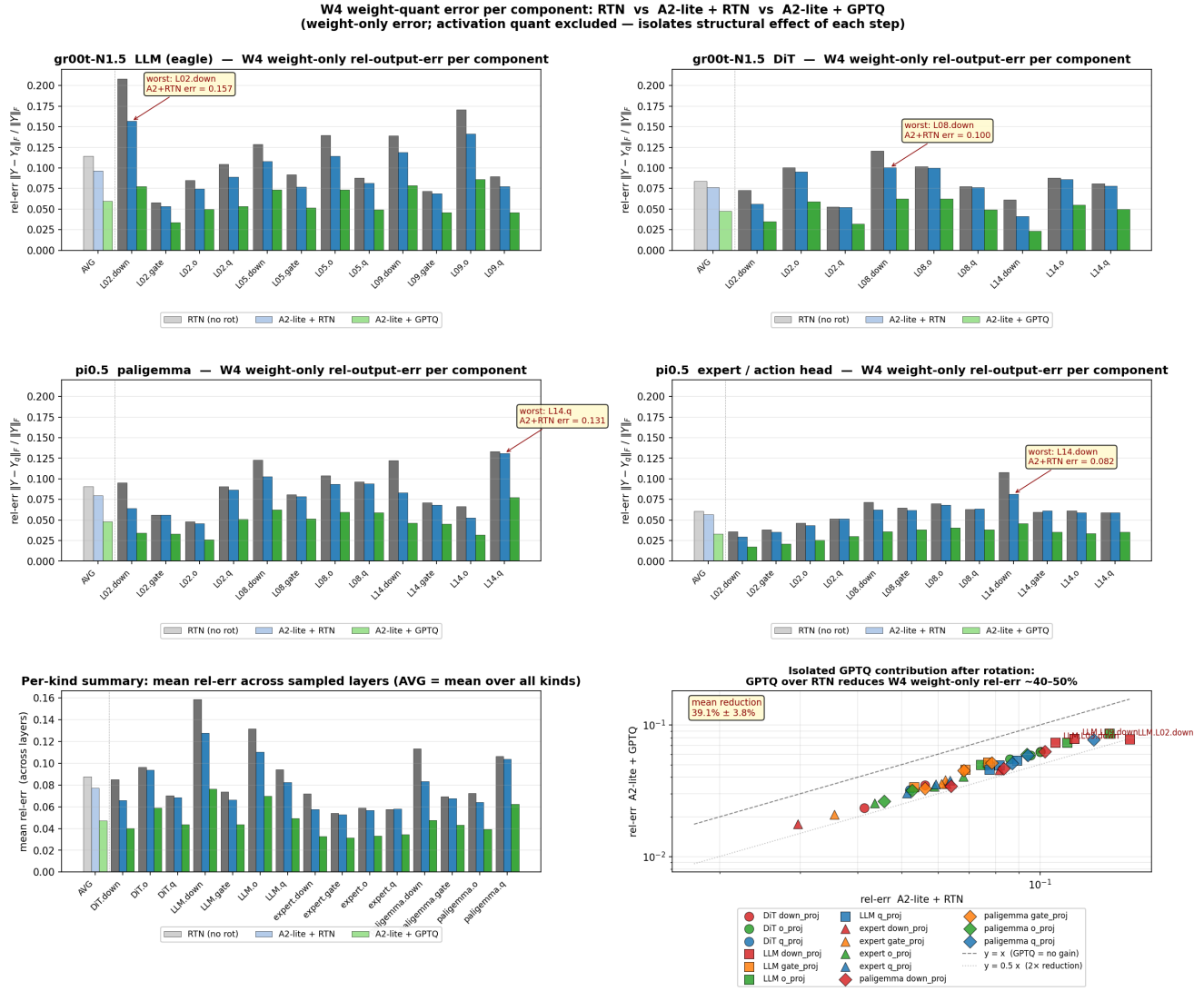
Figure 5: Per-component W4 weight quantization error across gr00t-N1.5 and Pi-0.5. Relative output error |XW^T - XR, Q(WR)^T|_F / |XW^T|_F measured layer-by-layer for three weight pipelines: RTN with no rotation, SVD-Hadamard rotation + RTN, and SVD-Hadamard rotation + GPTQ. Activation quantization is excluded so the bars isolate the structural contribution of each weight-quant step.
