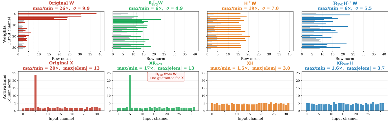
Figure 1: Per-channel distribution of weights (top) and activations (bottom) under four rotation settings. \mathbf{R}_{\text{SVD}} , adapted to \mathbf{W} , reduces the weight-row-norm spread substantially ( 26\times \rightarrow 6\times , \sigma: 9.9 \rightarrow 4.9 ), whereas the data-independent \mathbf{H} provides limited improvement ( 19\times , \sigma=7.0 ). Conversely, \mathbf{H} smooths activations ( 20\times \rightarrow 1.5\times ) via incoherence ( |(z\mathbf{H})_k| \approx \|z\|_2/\sqrt{n} ), while \mathbf{R}_{\text{SVD}} , derived entirely from \mathbf{W} , leaves activation outliers intact ( 20\times \rightarrow 17\times ). The composite \mathbf{R}_{\text{SVD}}\mathbf{H} inherits both strengths (weights: 6\times , \sigma=5.5 ; activations: 1.6\times ). These panels visualize the deterministic Hadamard \mathbf{H}_C ; the random signs \mathbf{D} in the full transform \mathbf{D}\mathbf{H}_C act as a worst-case incoherence safeguard against adversarially aligned inputs and are omitted here.
