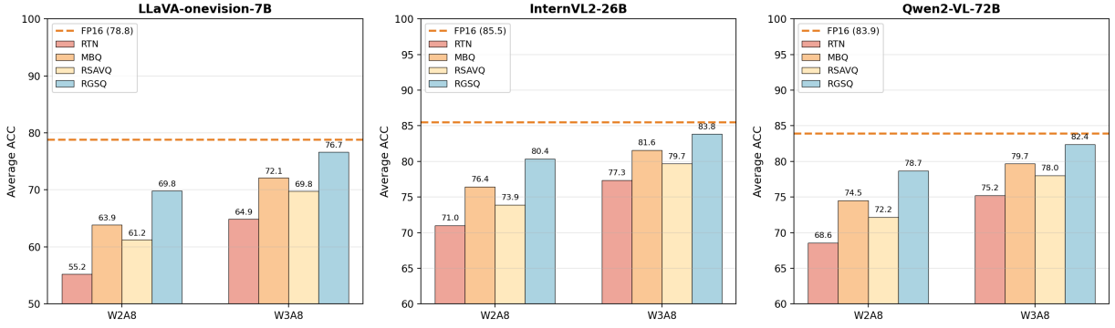
Fig. 3. Average performance across three benchmarks (ScienceQA, SEED, and TextVQA) under low-bit quantization settings (W2A8 and W3A8). RSAVQ is designed for LLMs and shows limited gains on VLMs, while MBQ and RGSQ are VLM-aware methods.
