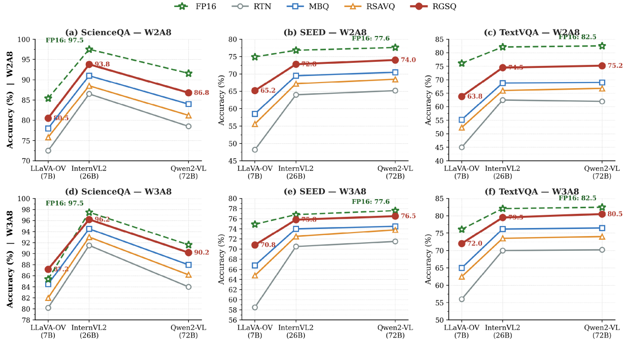
Fig. 4. Low-bit quantization results under W2A8 and W3A8 settings. RSAVQ is designed for LLMs and shows limited gains on MLLMs, while MBQ and RGSQ are MLLM-aware methods.
