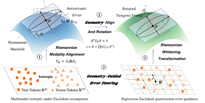
Fig. 1. Illustration of the RGSQ framework: Rather than assuming multimodal quantization error is Euclidean and isotropic, we characterize each layer with a modality-aware Riemannian metric that reveals anisotropic, loss-sensitive directions. RGSQ then applies geometry-aligned rotations to reorient the local tangent frame, steering low-bit perturbations toward low-sensitivity axes. Finally, Riemannian whitening maps the metric back to an equivalent Euclidean form, enabling plug-and-play use of standard PTQ solvers for efficient error scoring and optimization.
