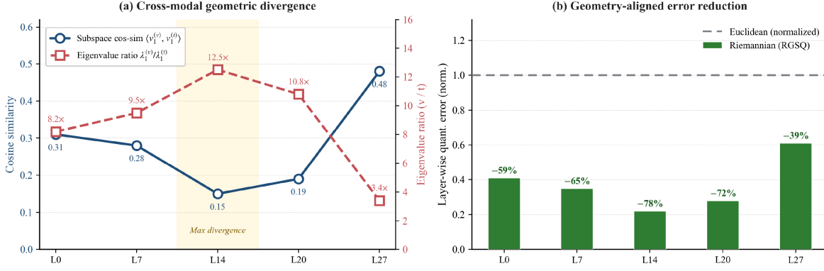
Fig. 5. Layer-wise geometric diagnostics on LLaVA-OneVision-7B under W4A8 quantization. We report modality eigenspace divergence and the corresponding reduction in normalized quantization error.
