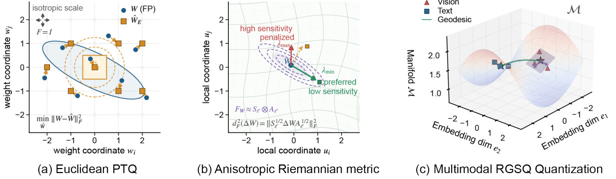
Fig. 2. Illustration of the key motivation: (a) Euclidean PTQ quantifies distortion using an isotropic \ell_2 metric, which fails to capture anisotropic sensitivity. (b) A Riemannian metric makes this anisotropy explicit through curvature-aware distortion, but incurs substantially higher computational cost. (c) The proposed RGSQ reconciles this trade-off in VLMs by building a modality-aware unified Riemannian geometry that aligns cross-modal distortion scales with practical overhead, and by steering low-bit perturbations toward loss-insensitive directions.
