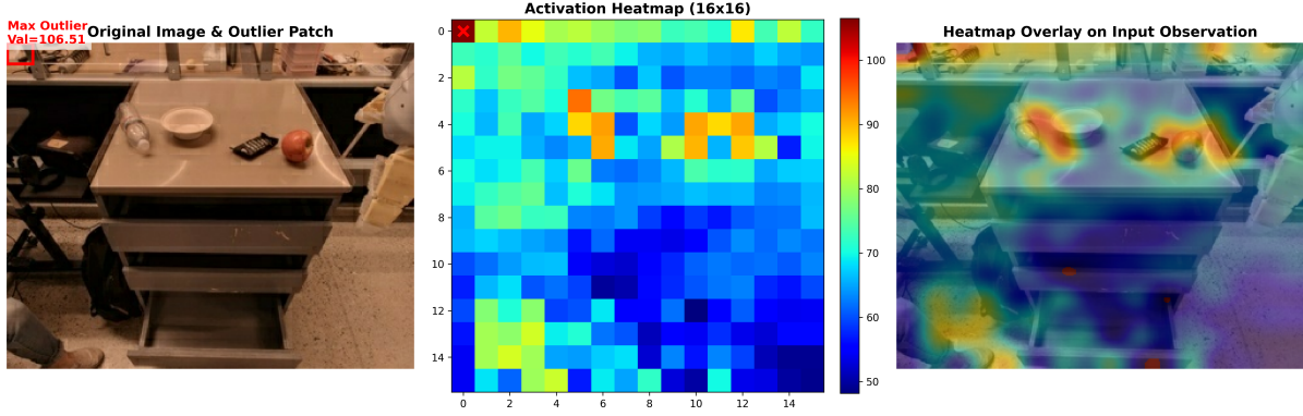
Figure 1: Left: An extreme background activation (Val=106.5). Middle: The activation heatmap is dominated by statistical outliers. Right: The overlay reveals misalignment: distractors such as the water bottle and background clutter dominate over the task-relevant apple, illustrating the dual-dominance problem.
