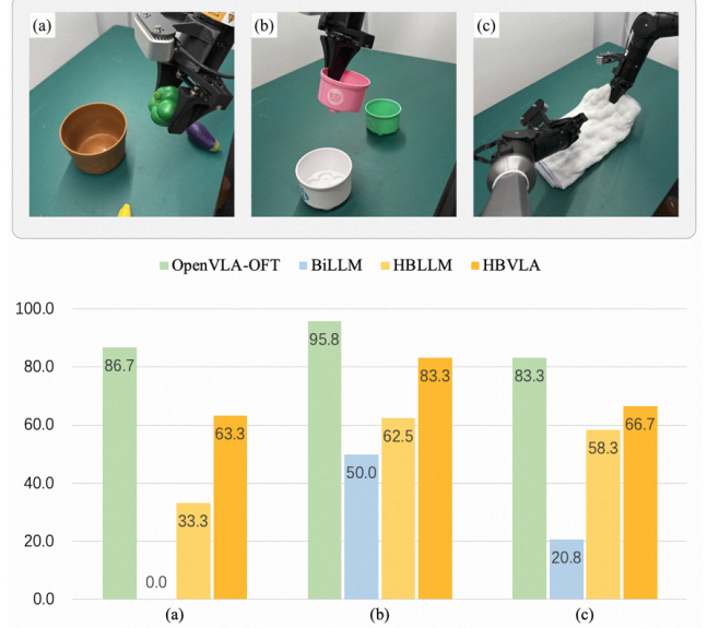
Figure 3: Comparison of baseline methods on the Mobile ALOHA experiments. Evaluation across three real-world tasks, including (a) Pick and Place, (b) Sequenced Instruction, (c) Flexible Folding. Top: Middle state image for each task. Bottom: Task-specific success rates for OpenVLA-OFT (FP Model), our HBVLA method, and baselines, including BiLLM and HBLLM.
