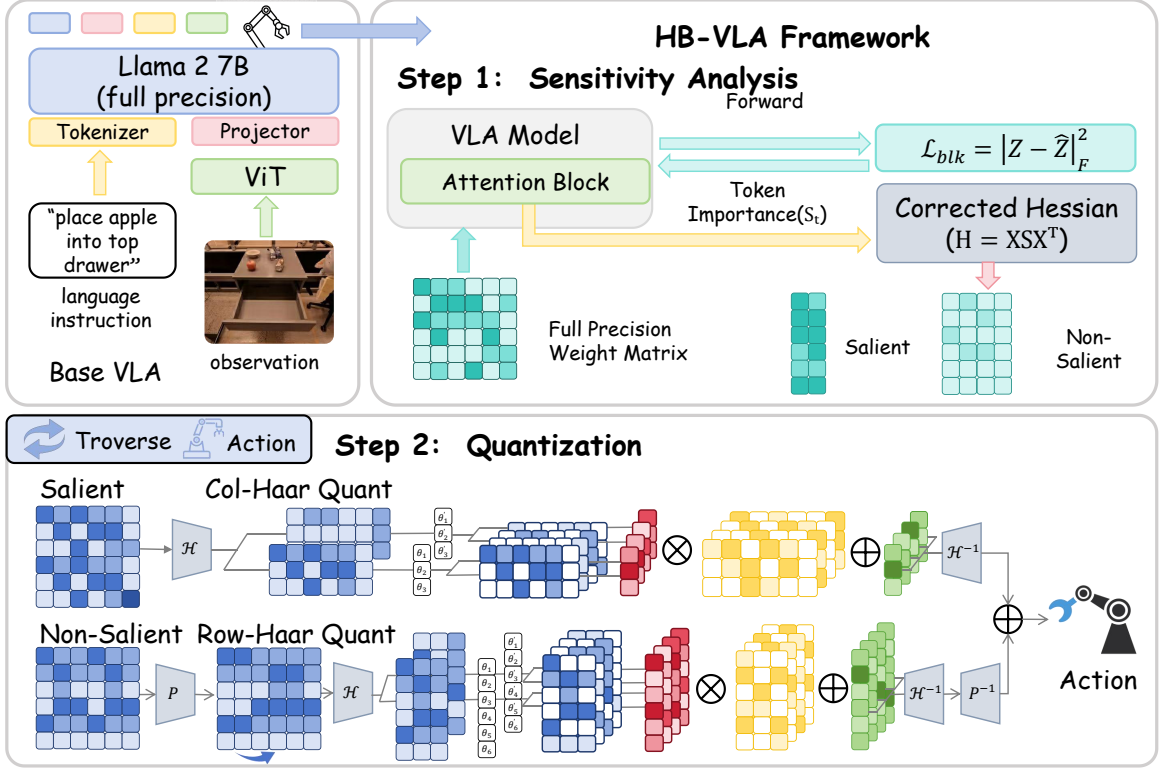
Figure 2: (i) We establish a block-wise gradient probe to derive token importance scores ( S_t ) and construct a Corrected Hessian proxy to identify functionally salient weights grounded in the policy. (ii) We apply a hybrid quantization strategy: salient weights undergo residual quantization, while non-salient weights are processed via sparse orthogonal transform ( P ) and Haar wavelet transform ( \mathcal{H} ) prior to group-wise 1-bit quantization.
