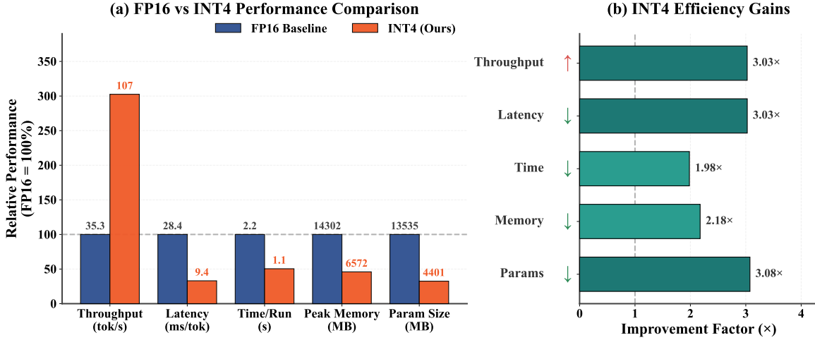
Figure 7. Deployment efficiency comparison between LLaVA-1.5 7B FP16 and GRACE 7B INT4 on A100 GPU. (a) Performance metrics normalized to FP16 baseline (100%). (b) Improvement factors achieved by INT4 quantization.
