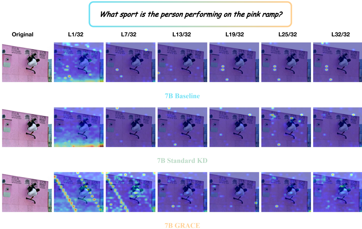
Figure 11. Multi-layer attention visualization for the question “What sport is the person performing on the pink ramp?” Standard KD produces attention patterns similar to the baseline, while GRACE progressively focuses on the task-relevant skateboard region.
