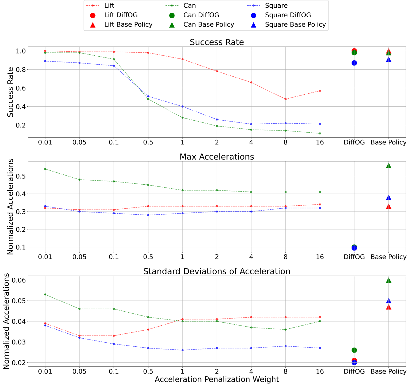
Fig. 13: Residual policy training with varying smoothness penalty weight \alpha .
