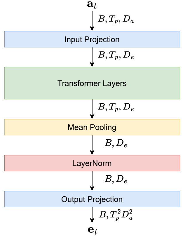
Fig. 3: Pipeline of the transformer encoder.
