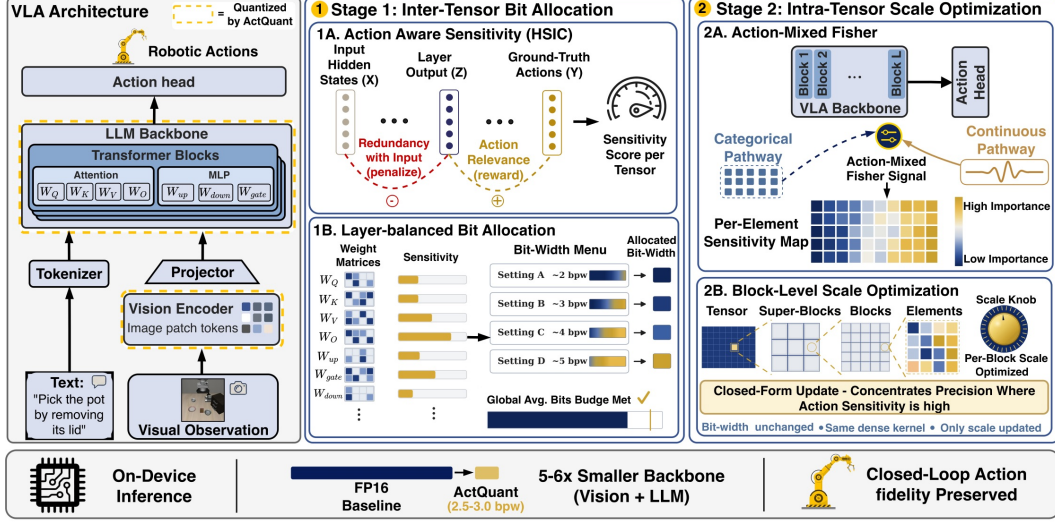
Figure 2: Overview of ActQuant. Stage 1 (inter-tensor): an action-aware HSIC sensitivity score assigns each matrix a single bit-width under a budget. Stage 2 (intra-tensor): with the bit-width fixed, the per-block scales within each matrix are optimized, weighted by per-element sensitivities from an Action-Mixed Fisher that combines the action-head loss with an optional LM loss.
