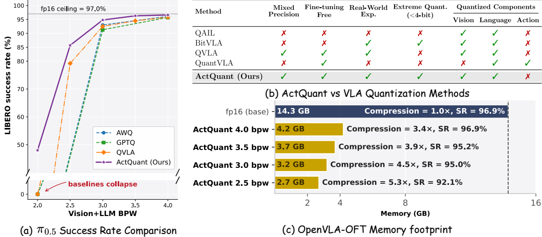
Figure 1: (a) Average success rate on LIBERO ( \pi_{0.5} ) as the backbone bit-width drops from 4.0 to 2.0 bpw. (b) Comparison of ActQuant with other VLA quantization methods. (c) Backbone memory usage across average bit-widths, with compression ratio against the baseline and success rate (SR).
