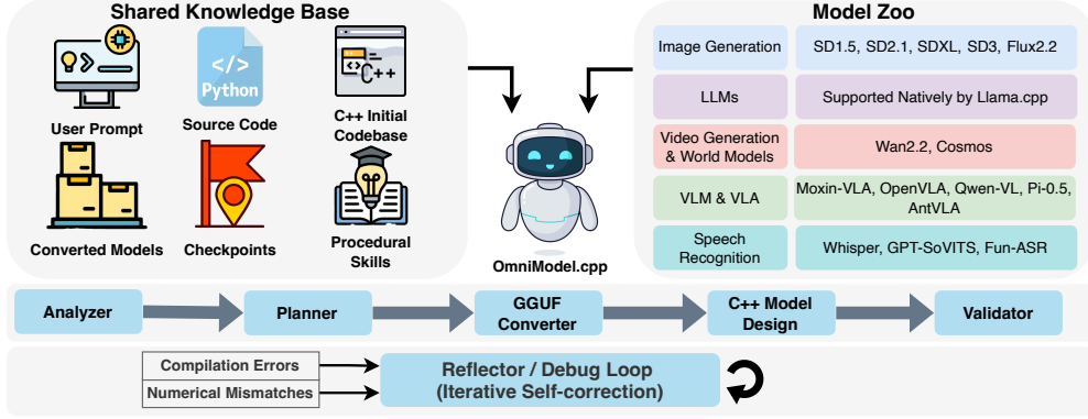
Figure 4: OmniModel.cpp pipeline for deploying ActQuant-quantized VLA backbones in native C/C++. A shared knowledge base and a library of procedural skills feed a planner-driven loop (analyze, plan, convert to GGUF, build the GGML graph, validate); a reflector iterates on compilation errors and per-tensor numerical mismatches against the PyTorch reference until parity is reached.
