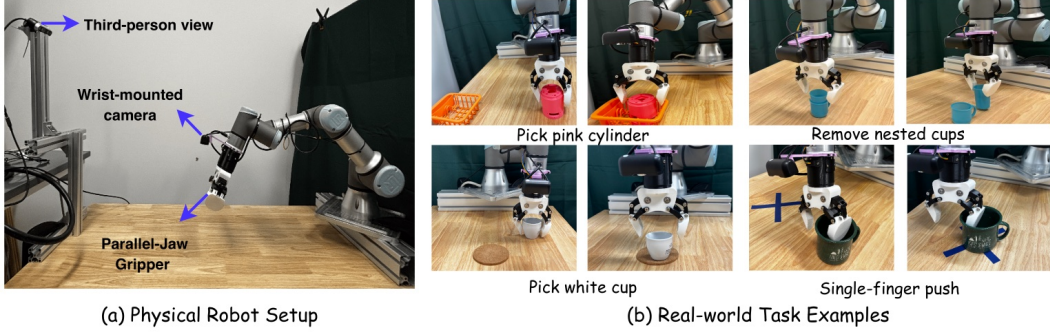
Figure 3: Physical robot setup and real-world task demonstrations. The system consists of a UR3 robot arm, wrist-mounted camera, and third-person view camera.
