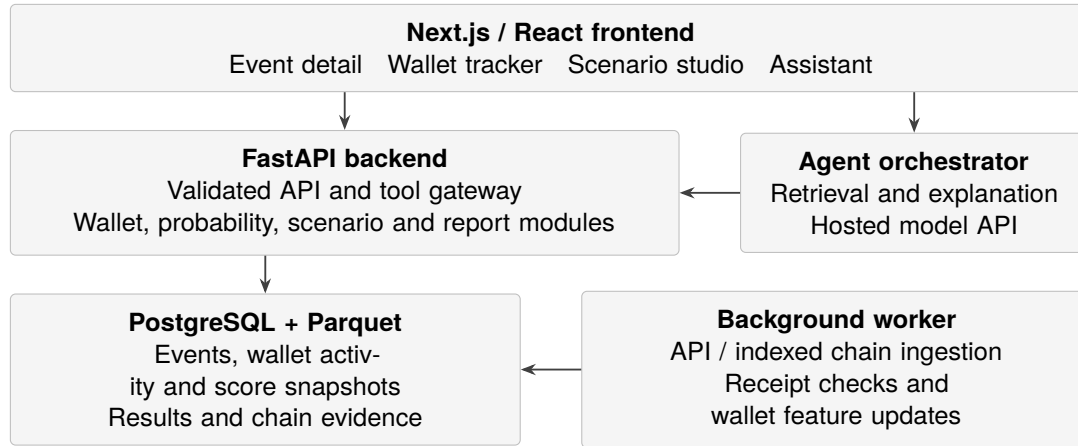
Figure 6: Proposed application architecture. The dashboard and assistant share the same calculation services and stored results.
