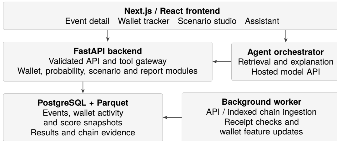
Figure 5: Proposed application architecture. The dashboard and assistant share the same calculation services and stored results.
