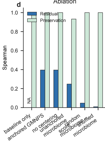
Ablation
