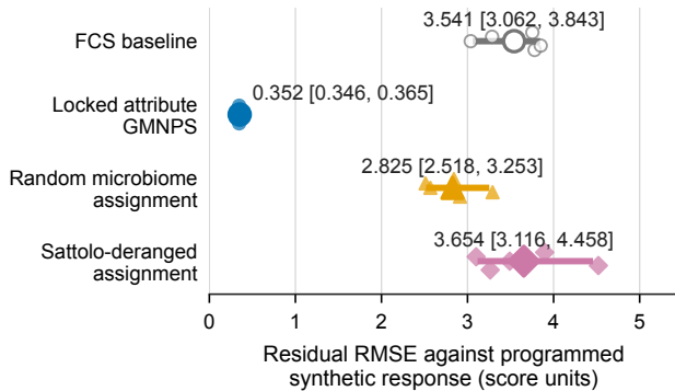
a Programmed residual error
