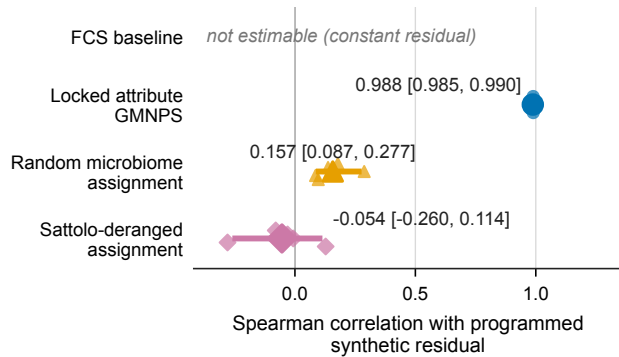
b Programmed residual rank recovery
