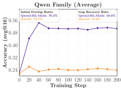
— Qwen3-4B-Non-Thinking-RL-Math — Qwen3-4B (Non-thinking)
