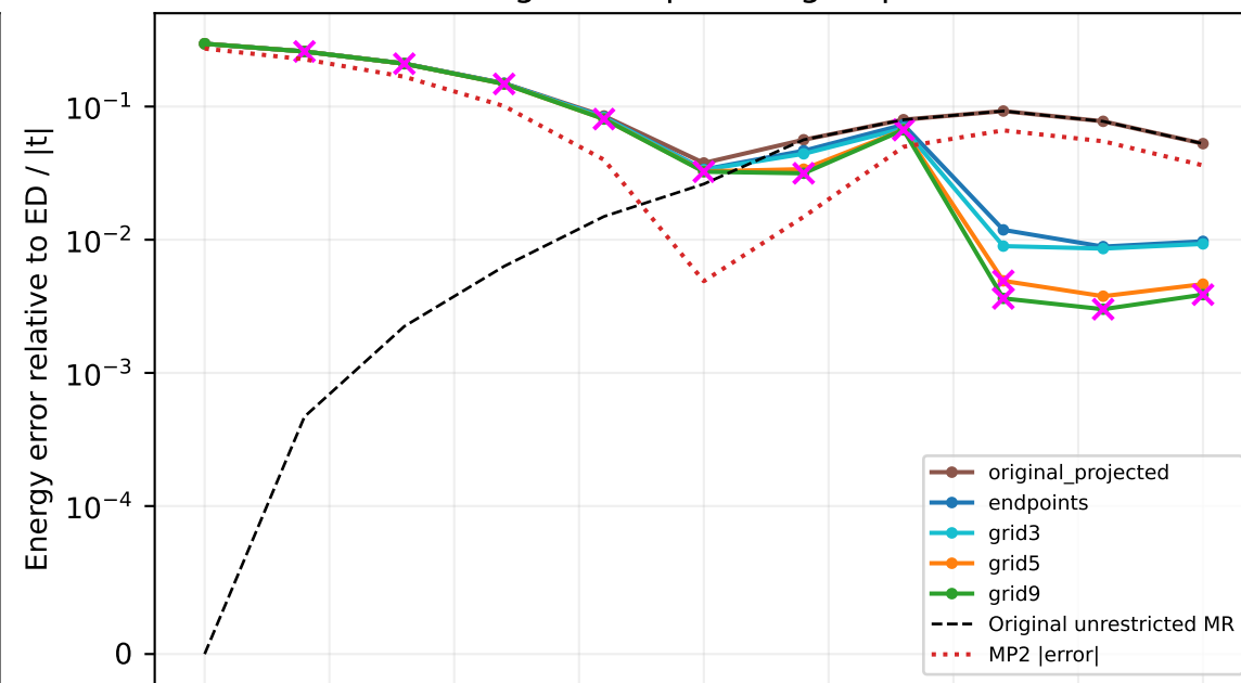
\omega=5 : equal-weight q=+1
