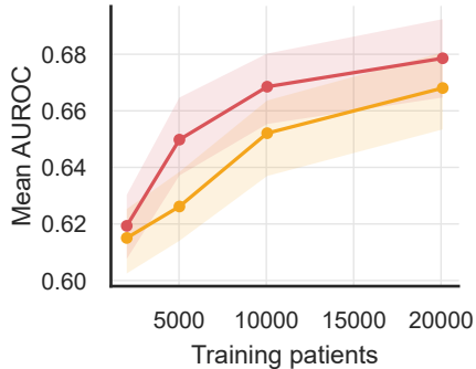
A Training: MIMIC-IV; held-out MIMIC-IV
