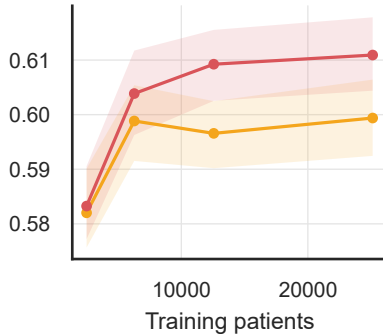
B Training: MIMIC-IV; test: MIMIC-III
