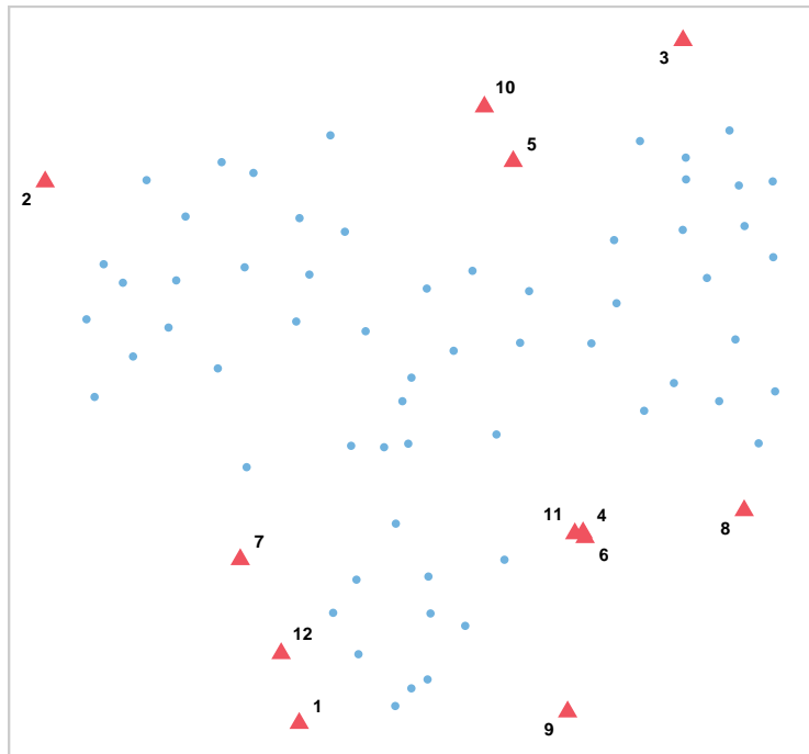
archetypes_umap_CAF
