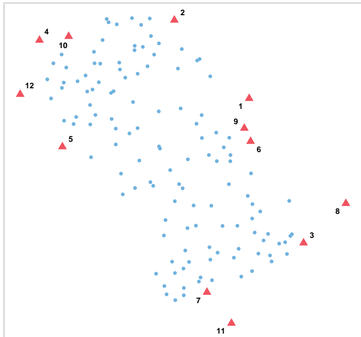
archetypes_umap_Macro
