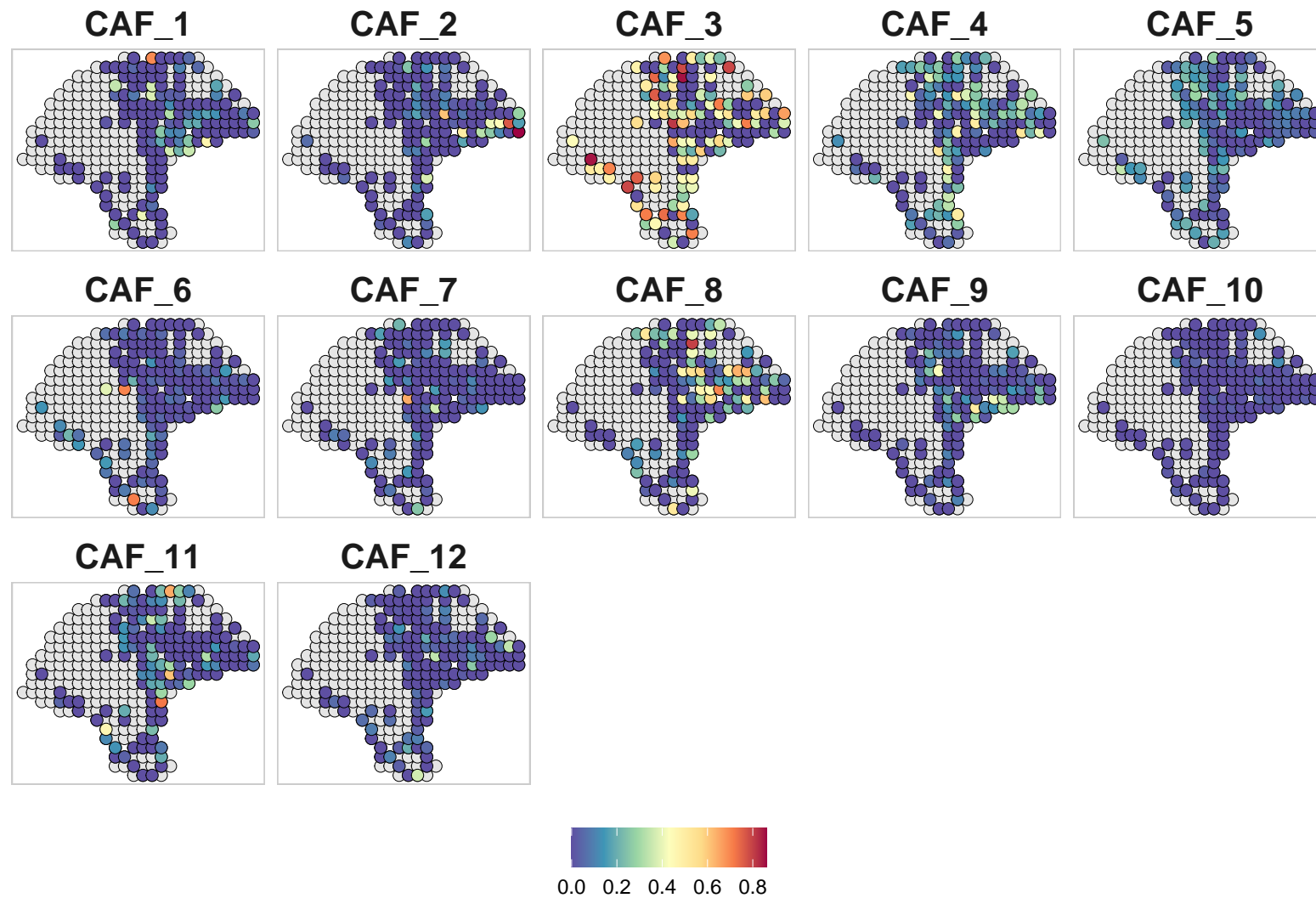
CAF_alpha_heatmap
