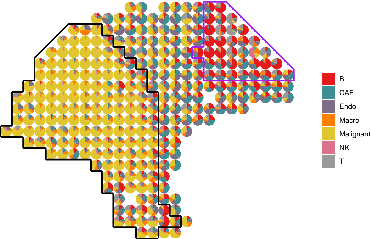
segmentation_lymphoid_melanoma
