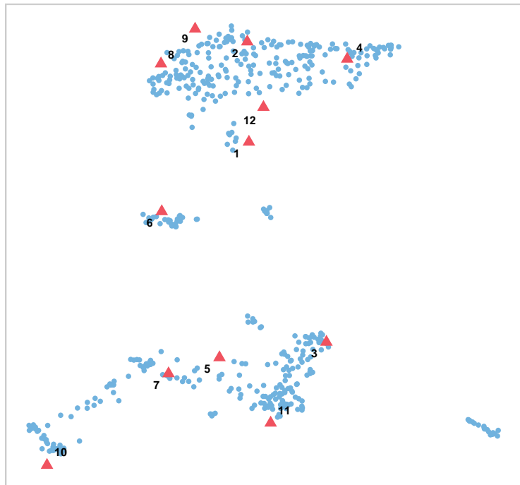
archetypes_umap_Malignant
