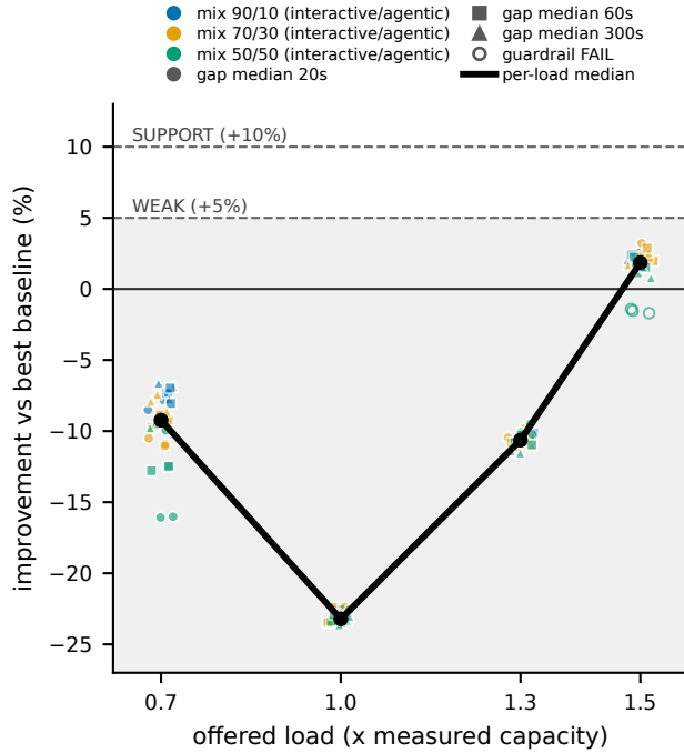
Figure 3. Per-cell improvement of the reservation discipline over the best per-cell tuned baseline, across offered load. Each point is one of 108 pre-registered core cells; the heavy line traces the per-load median. The deficit is U-shaped, deepest at nominal provisioning (22.4 to 23.6 percent at 1.0x), and the sign flips past saturation (+0.8 to +3.2 percent at 1.5x). Dashed lines mark the pre-registered WEAK (+5 percent) and SUPPORT (+10 percent) thresholds; no cell reaches SUPPORT. Open symbols mark the four cells failing the interactive guardrail (Section 6.4).
