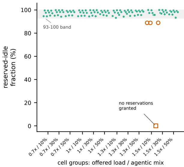
Figure 6. What that isolation costs. Reserved-idle fraction per cell: the protection of Figure 5 is priced in capacity held idle, 93 to 100 percent of the reserved pool in 77 of 81 cells, with three load-1.5 cells at 88.9 percent and one cell granted no reservations (marked). This is the structural duty-cycle cost of Section 6.5.
