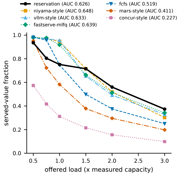
Figure 4. Served value across the load sweep. The reservation discipline's area under curve (0.626) trails deadline-ordered class scheduling (0.648), killing the graceful-degradation hypothesis; the admission-throttling baselines collapse under overload (Section 6.5).
