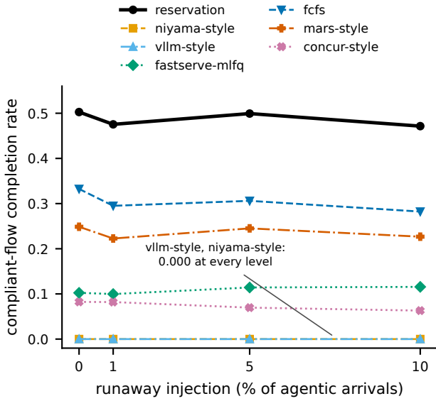
Figure 1. Compliant-flow completion under adversarial runaway injection, absolute rates. The reservation discipline holds near 0.5 with a worst-case degradation of 3.1 points; FCFS completes 0.33 with no containment; the two strongest request-oriented baselines complete zero compliant flows at every level including no injection, instrumented admission starvation (one of 107 compliant flows ever scheduled, zero preemptions; Section 6.1). Deltas against zero are undefined, which is why rates are absolute.
