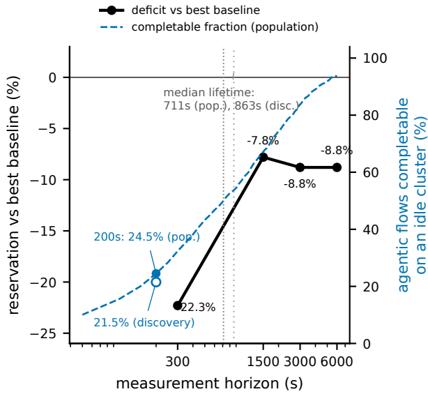
Figure 2. Horizon censoring on one core cell. The population median agentic flow lifetime, derived from the released workload generators, is roughly 711 seconds (first measured at 863 seconds on the diagnostic realization that surfaced the artifact, open markers); at a 200-second window only about a quarter of agentic flows can complete even on an idle cluster (24.5 percent of the population; 21.5 percent of the diagnostic realization), while the campaign’s default horizons ran 150 to 300 seconds. The measured deficit is 22.3 percent at a 300-second horizon and halves to 7.8 percent at adequate horizons, stable through 6000 seconds. Horizons shorter than the workload’s completable lifetimes charge guarantee-holders full stranding cost against zero completion payoff (Section 6.2).
