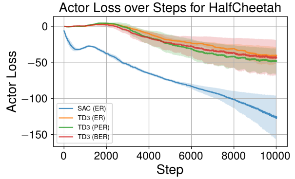
Figure 13: Actor Loss over the environment steps
