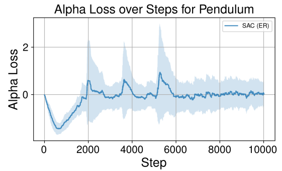
Figure 7: Alpha Loss over the environment steps
