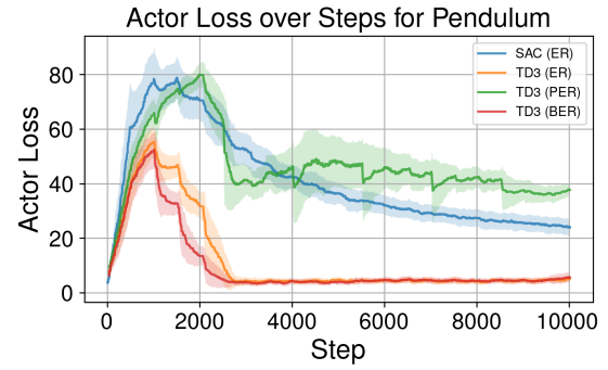
Figure 5: Actor Loss over the environment steps
