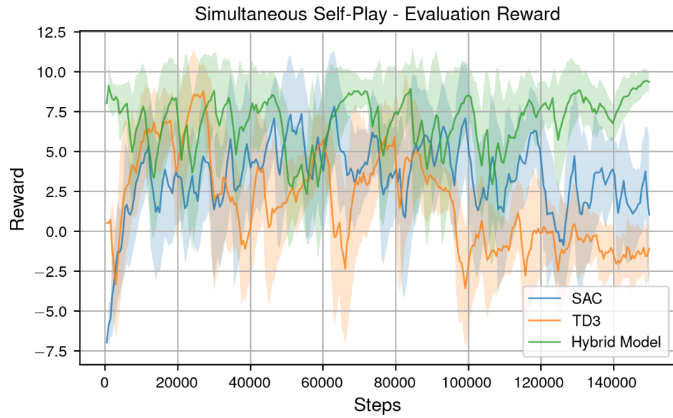
Figure 21: Selfplay Rewards Evaluation for SAC, TD3 and the Hybrid model.
