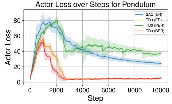
Figure 6: Actor Loss over the environment steps
