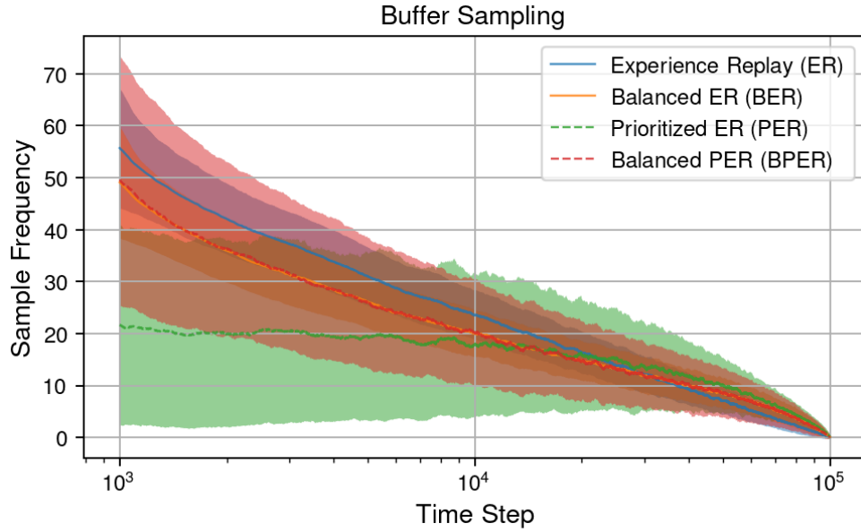
Figure 1: Sample frequency of the experiences for ER, BER, PER and BPER. The X-axis is displayed in log scale and the plot contains the moving average and confidence interval with a window size of 1000.
