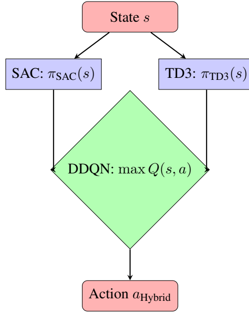
Figure 2: Hybrid-Model with DDQN Selection Gate
