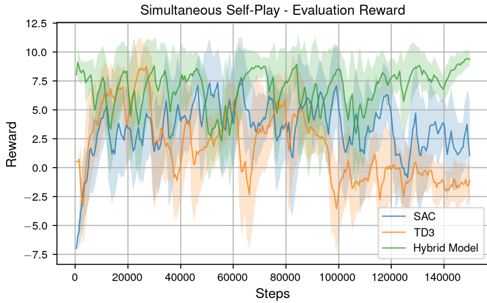
Figure 19: Selfplay Rewards Evaluation for SAC, TD3 and the Hybrid model.
