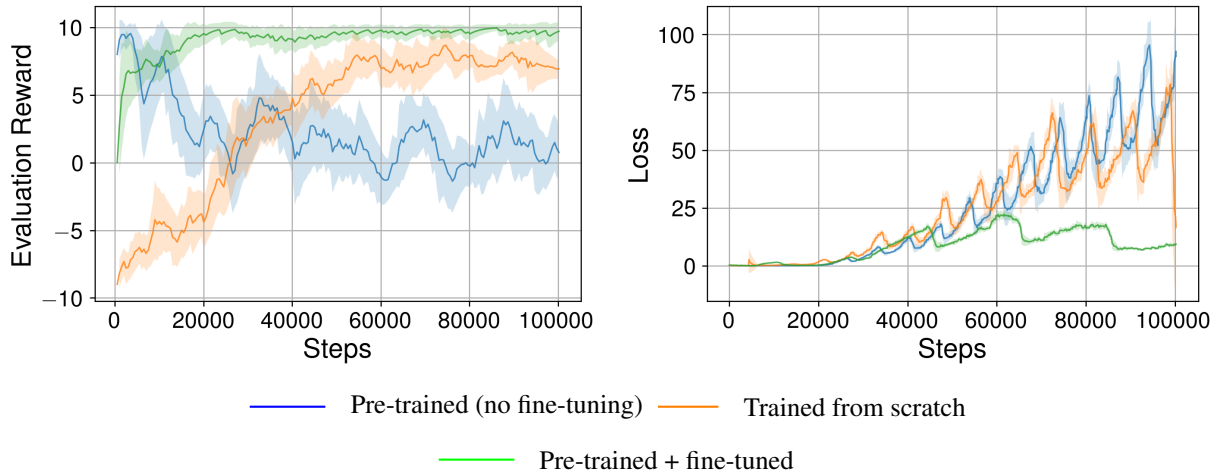
Evaluation reward and loss comparison of hybrid model training strategies
