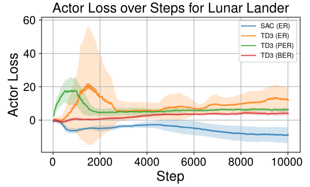
Figure 8: Actor Loss over the environment steps
