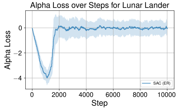
Figure 10: Alpha Loss over the environment steps
