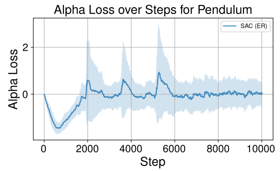
Figure 6: Alpha Loss over the environment steps
