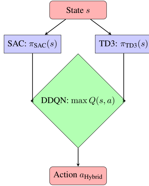
Figure 2: Hybrid-Model with DDQN Selection Gate
