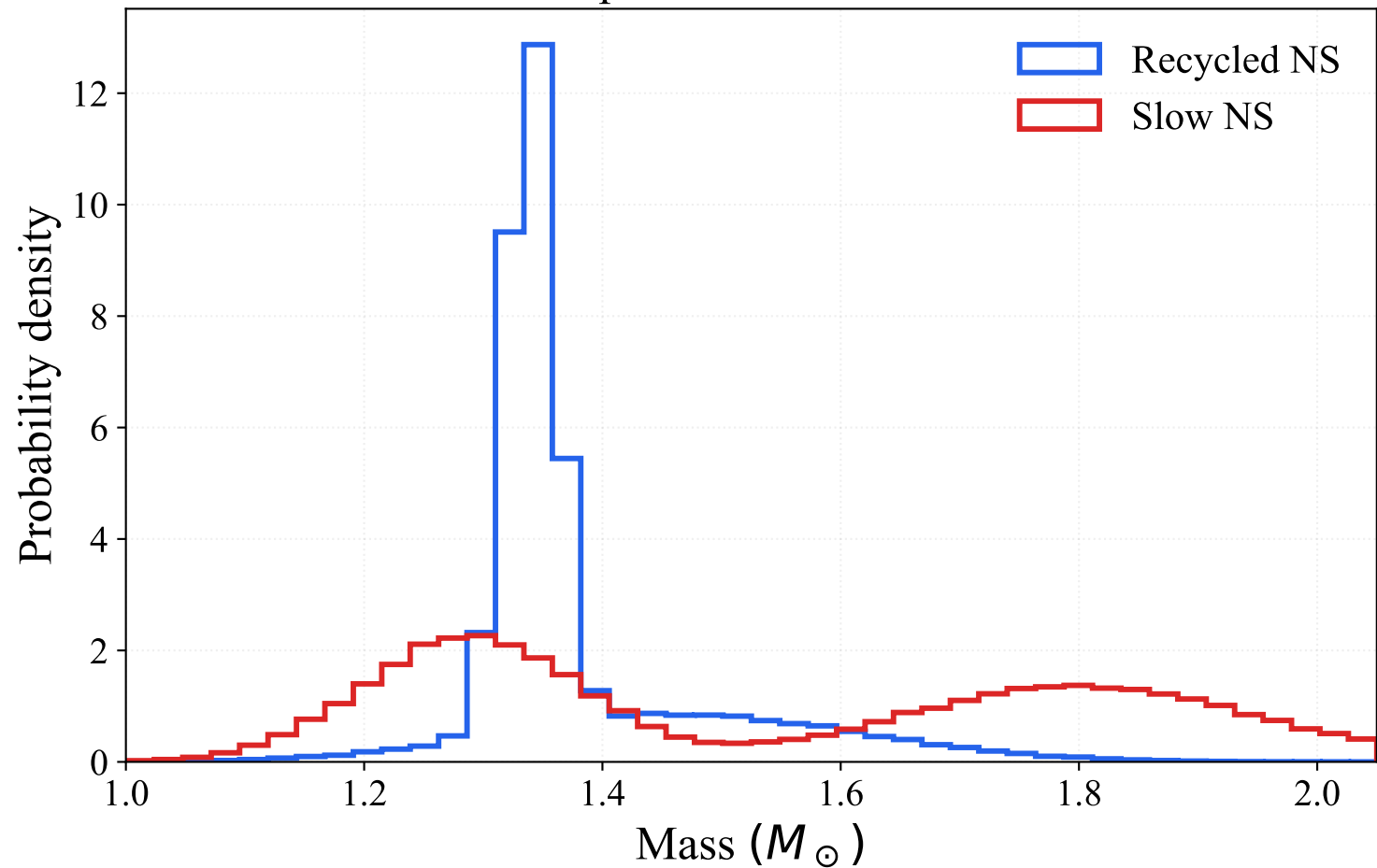
BNS Component Mass Distributions
