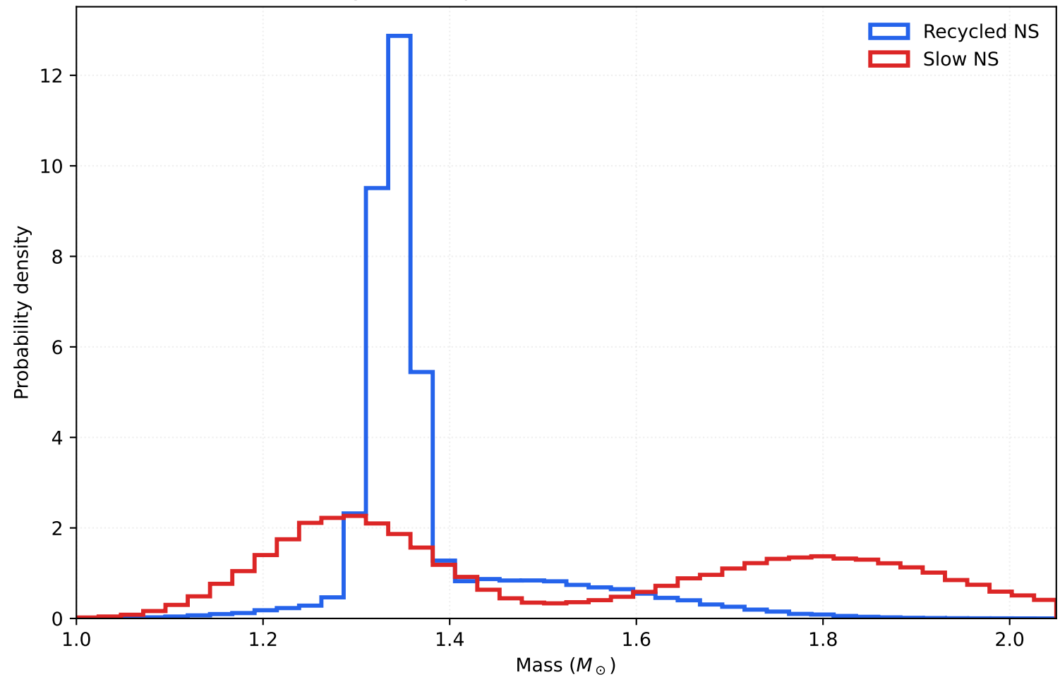
BNS Original Component Mass Distributions (Test Set)
