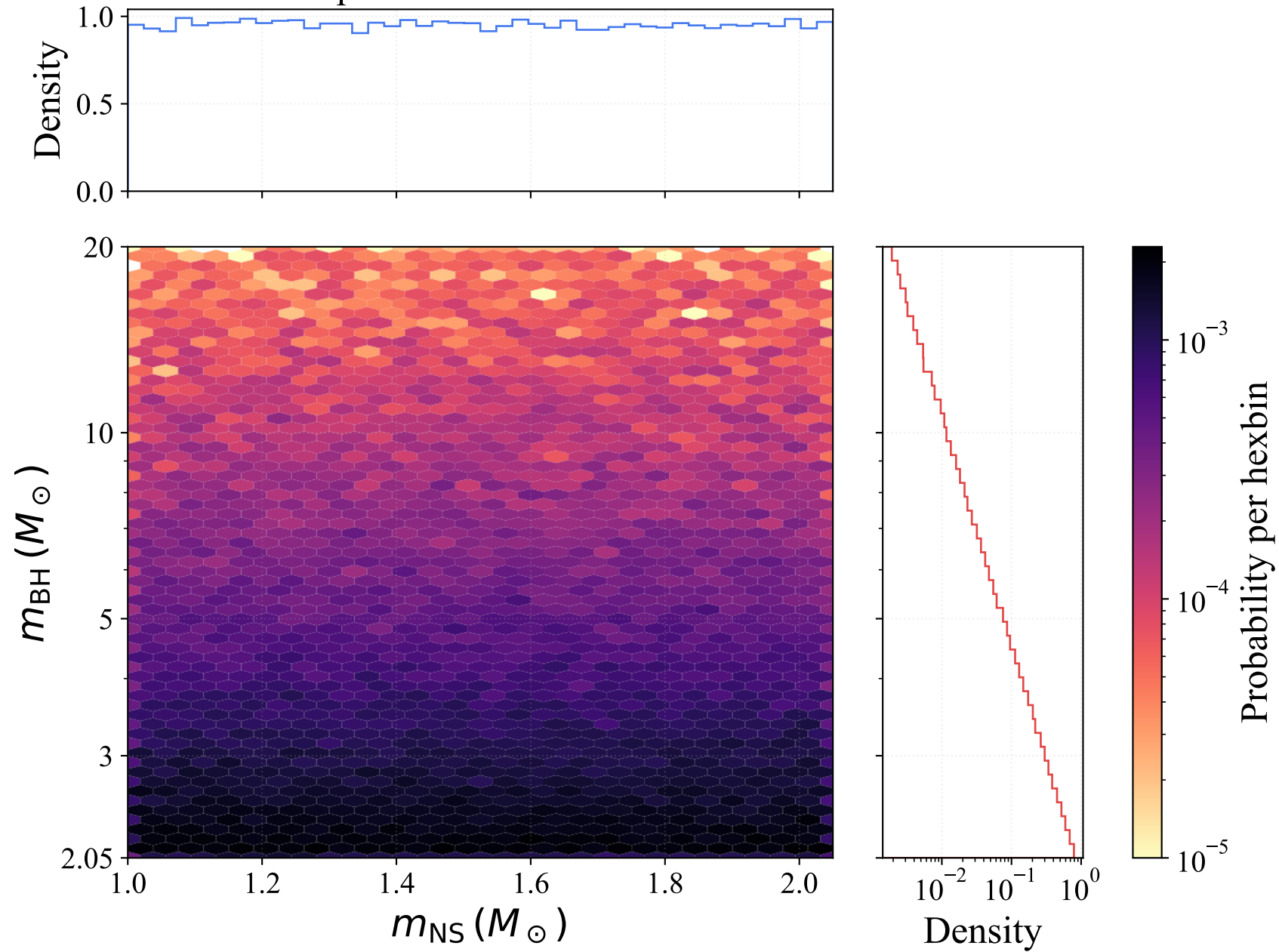
NSBH Component Mass Joint Distribution
