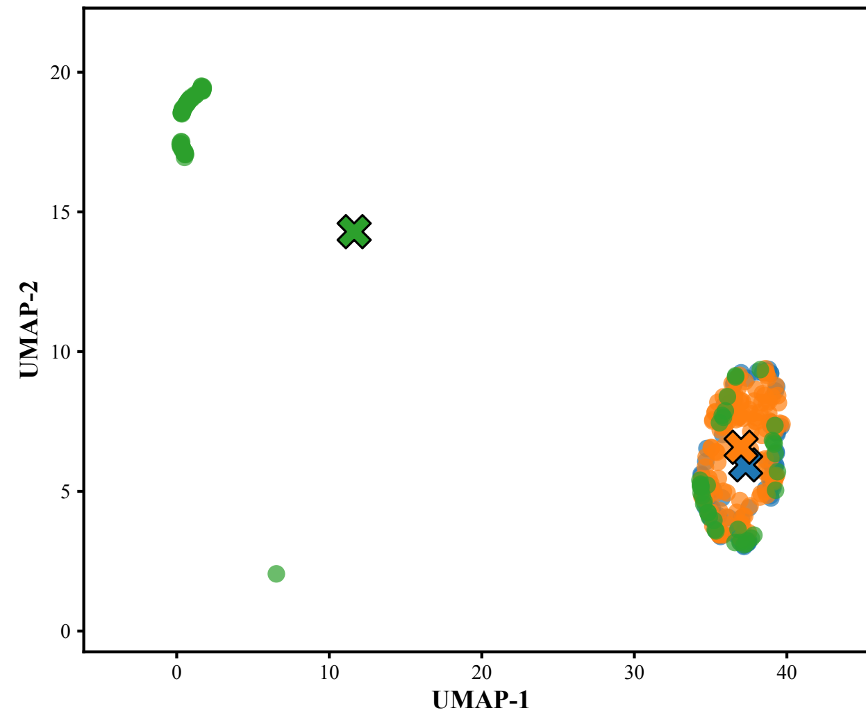
Koopman Component Silhouette = 0.093
