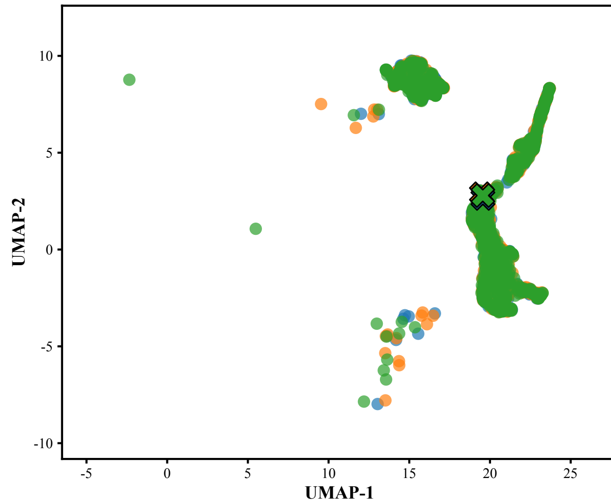
Koopman Component Silhouette = -0.012
