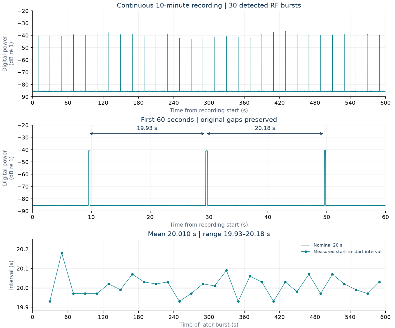
Figure 1. Continuous 600-second reception, including the original intervals without a beacon. Power is averaged over consecutive 10 ms windows of the original 192 ksamples/s complex channel; no amplitude normalization is applied. A threshold 20 dB above median recording power detects 30 RF bursts and 29 start-to-start intervals. Thresholds of 15 and 25 dB also give 30 bursts. Times lie on a 10 ms detection grid. These are energy detections, not counts of decoded packets or exact transmitter scheduling timestamps.
