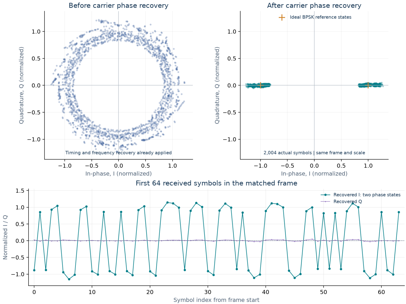
Figure 2. Actual mode 02 symbols before and after the order-2 Costas carrier phase recovery loop. Each point is one symbol. Both views use the same 2,004 symbols of the complete matched, HDLC-stuffed frame including FCS, with one shared RMS amplitude scale. No additional phase rotation or point removal is applied. Silence and preamble are outside this frame selection. The source WAV already includes its documented +870 Hz correction; timing and frequency recovery precede the left-hand trace.
