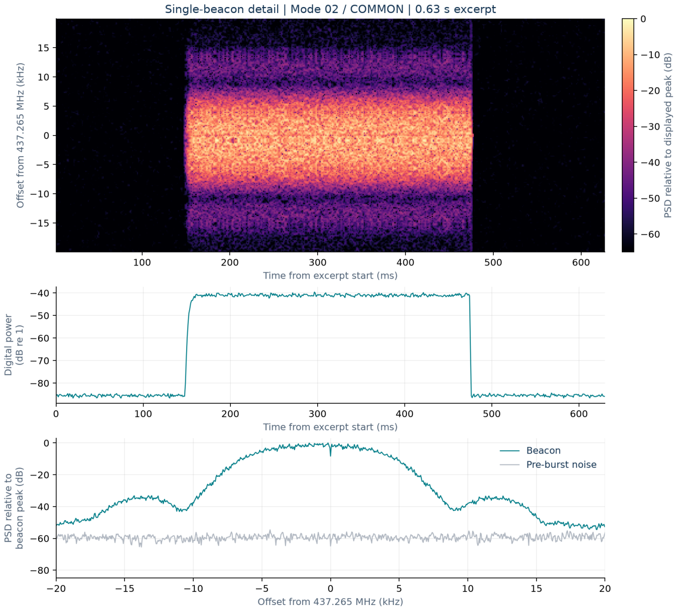
Figure 3. One mode 02 beacon in a 0.63-second excerpt; this view does not show the 20-second repetition interval. The plotted IQ is reconstructed from the supplied PCM WAV by reversing its documented amplitude scale and +870 Hz frequency correction. PCM quantization remains. Digital levels are not calibrated dBm. Waterfall: Hann window, 1,024 samples, 75% overlap; spectrum: Welch, 4,096 samples.
