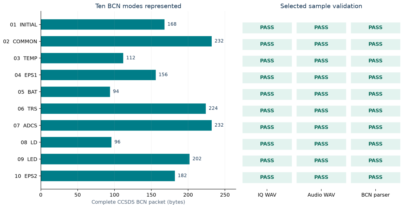
Figure 4. One selected example for each BCN mode. Both WAV formats independently reproduce the same CRC-verified AX.25 hex as the corresponding complex excerpt. All ten packets also pass the existing BCN parser. This is sample validation, not a packet reception rate.
