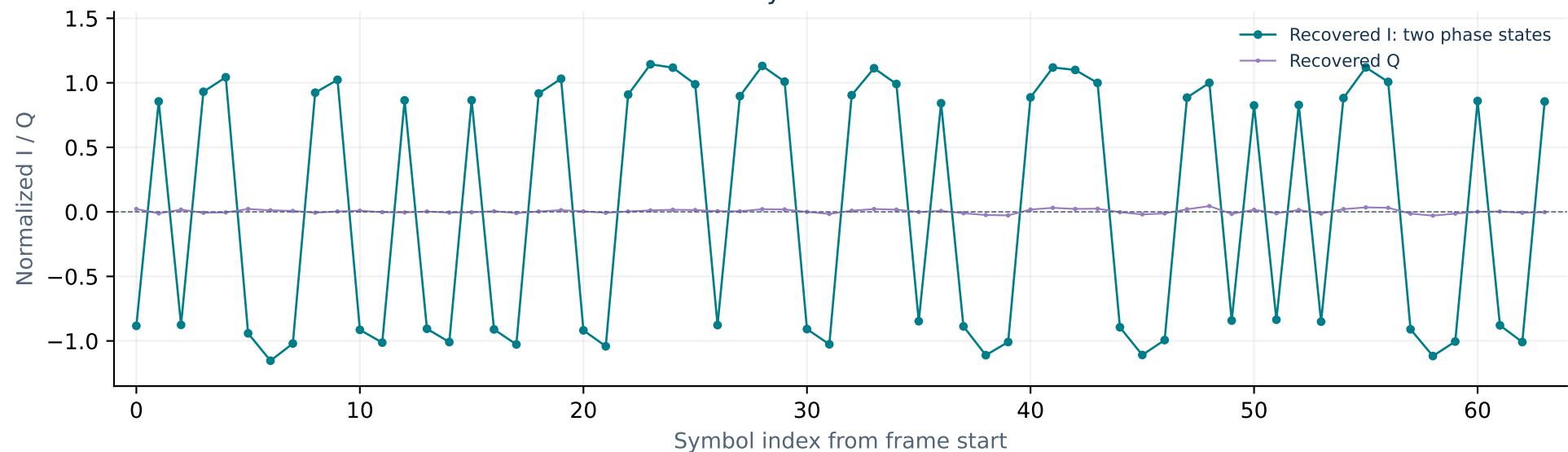
First 64 received symbols in the matched frame
