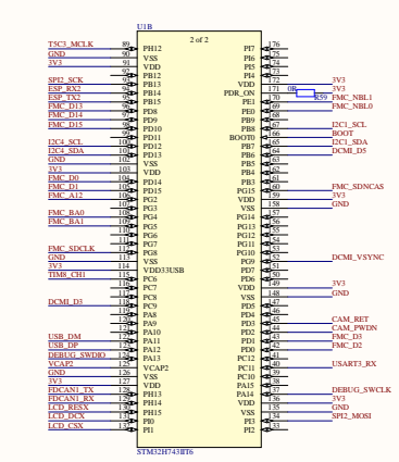
STM32H743IIT6
