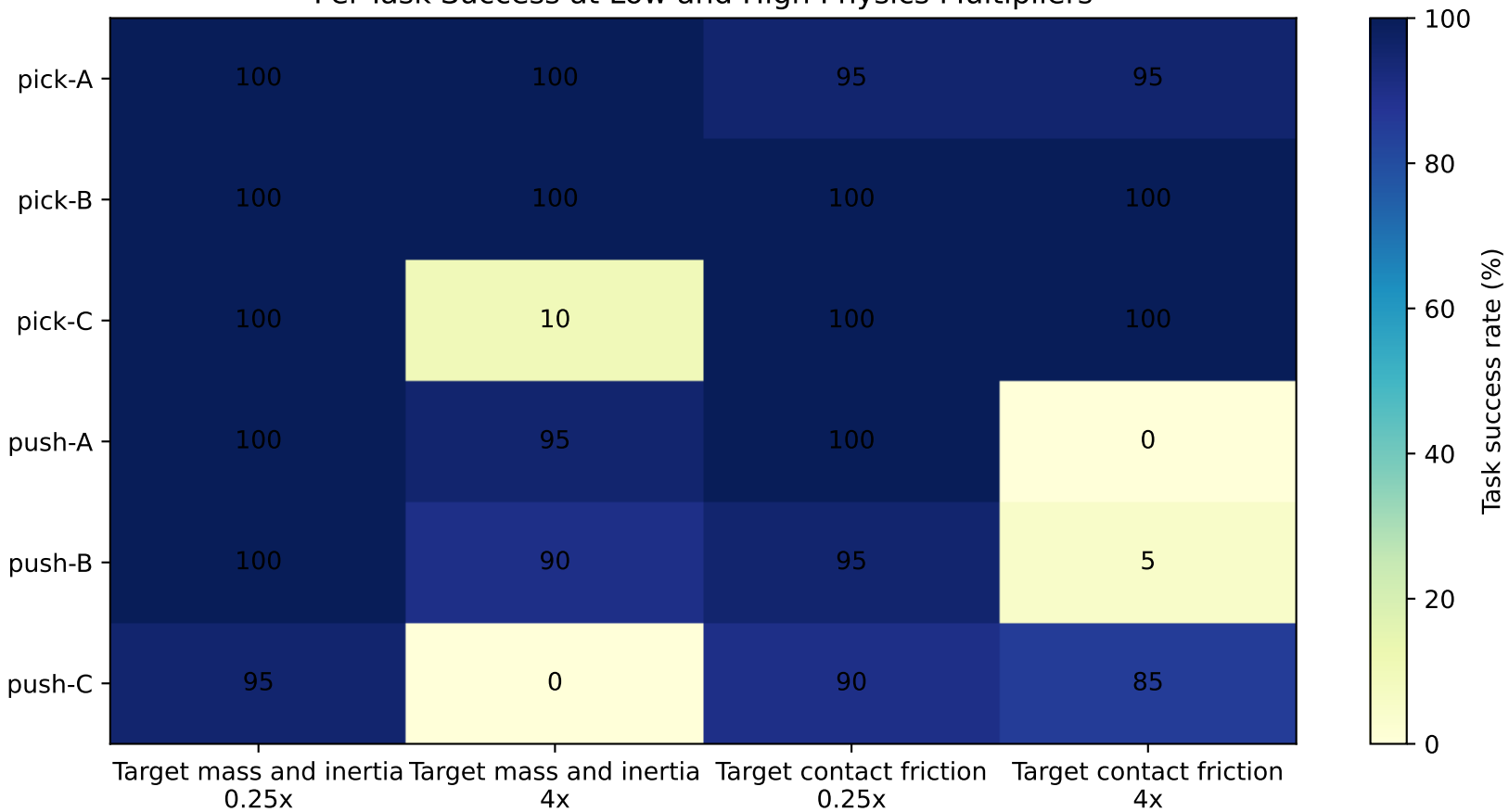
Per-Task Success at Low and High Physics Multipliers
