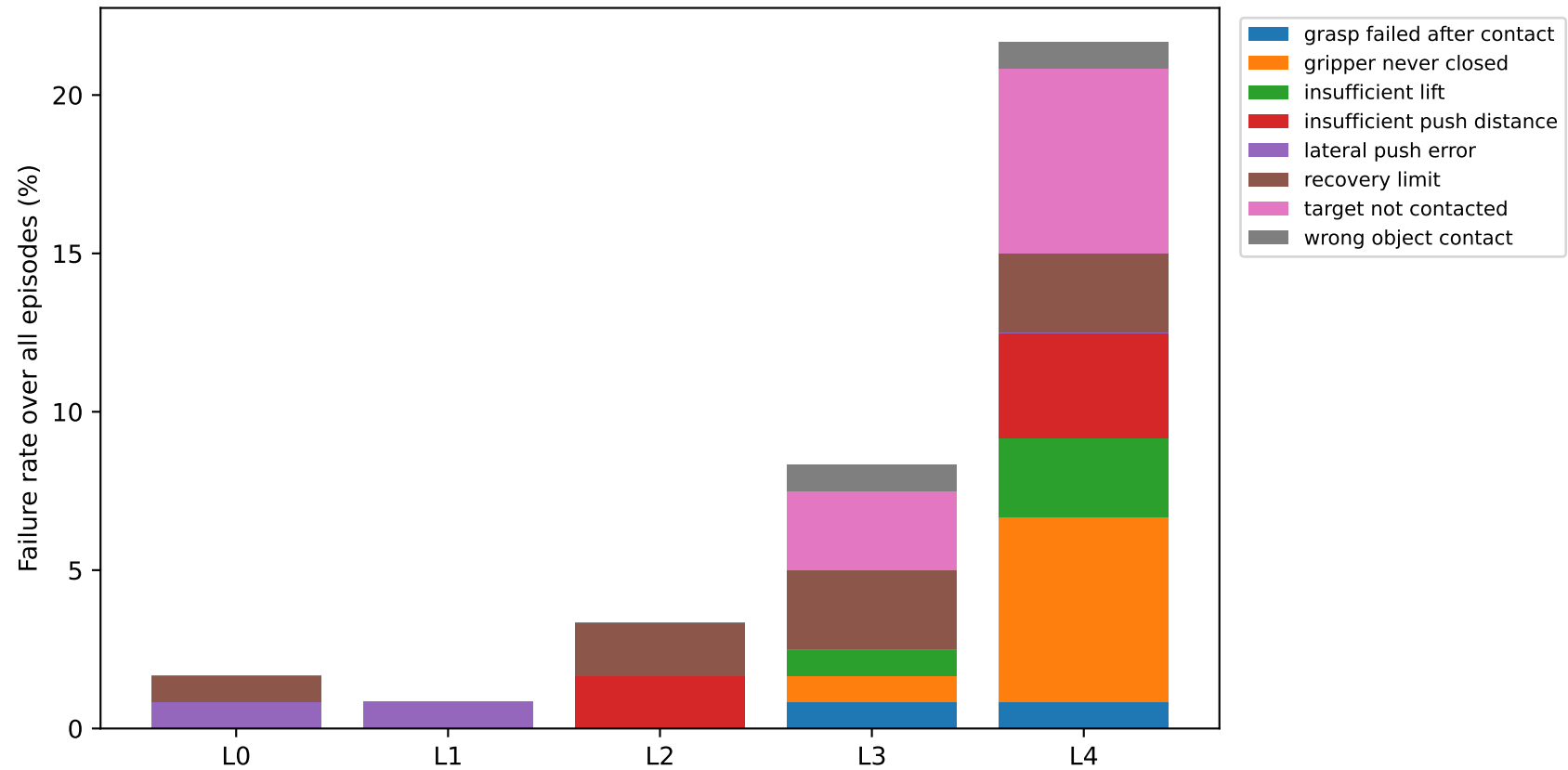
Failure Taxonomy Under Camera-Extrinsic Drift
