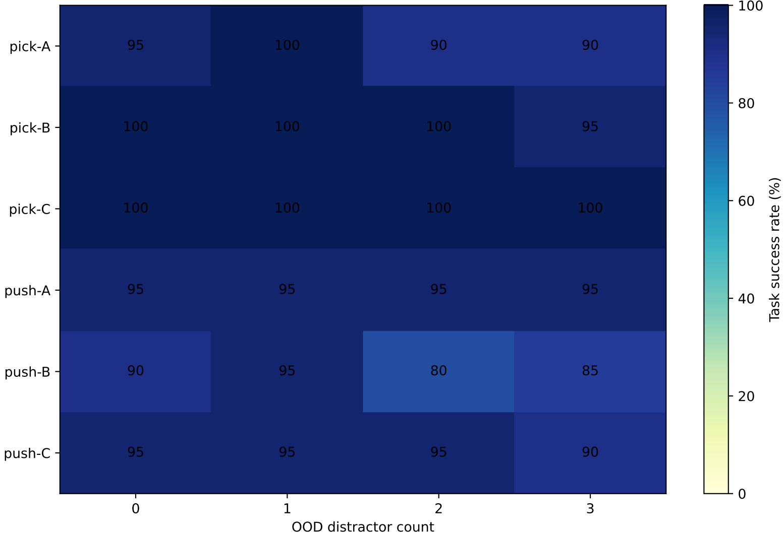
Per-Task Success Under OOD Distractors
