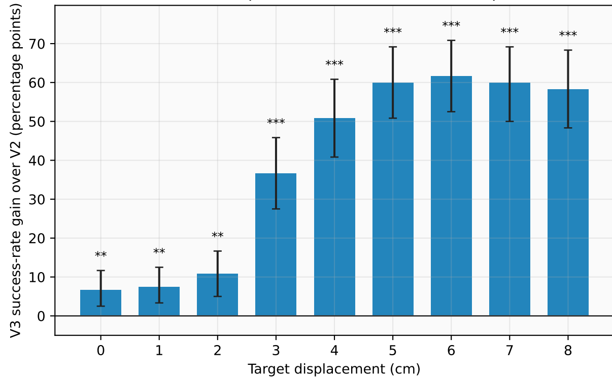
Paired V3 Improvement with 95% Bootstrap CI
