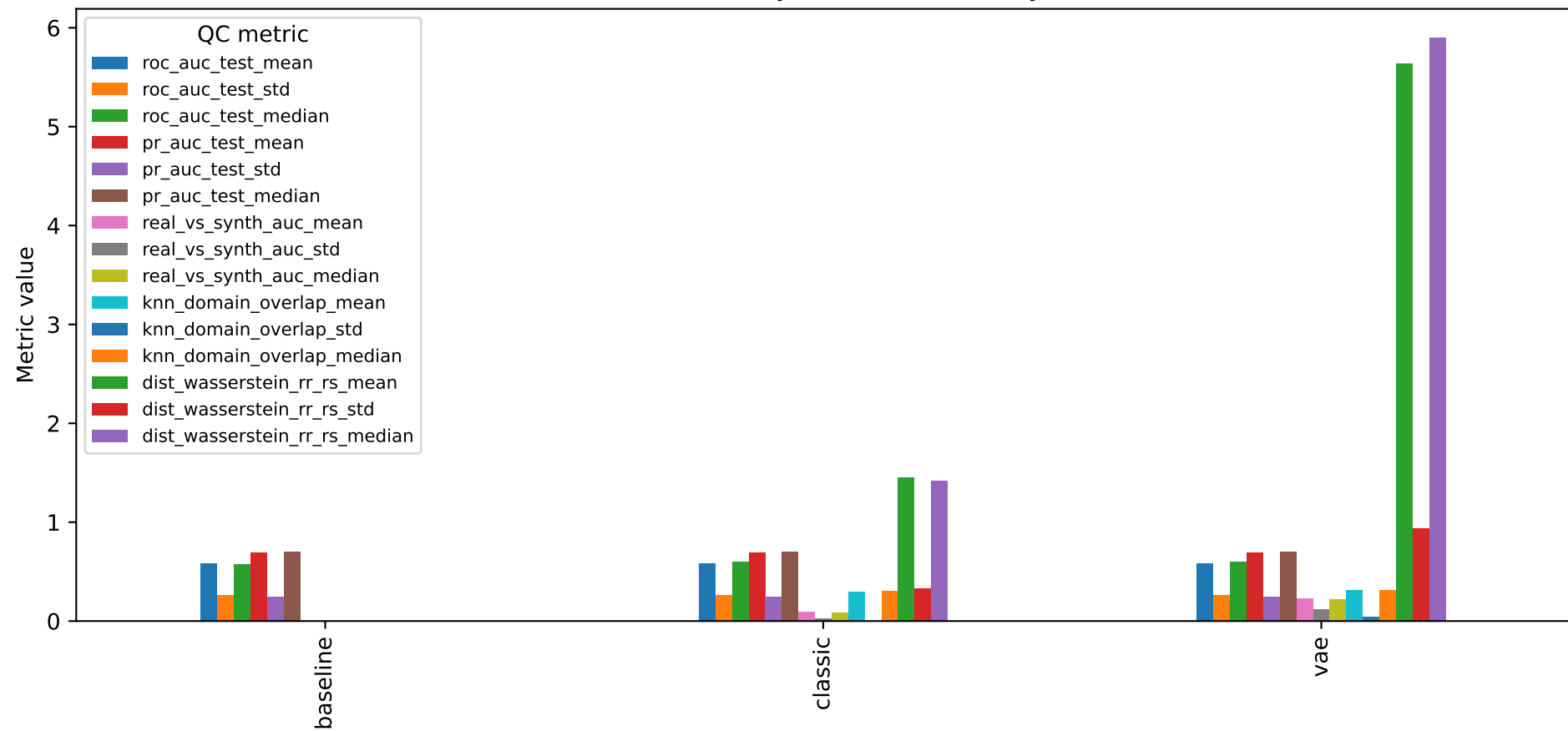
GDB broad window: synthetic-data QC by method
